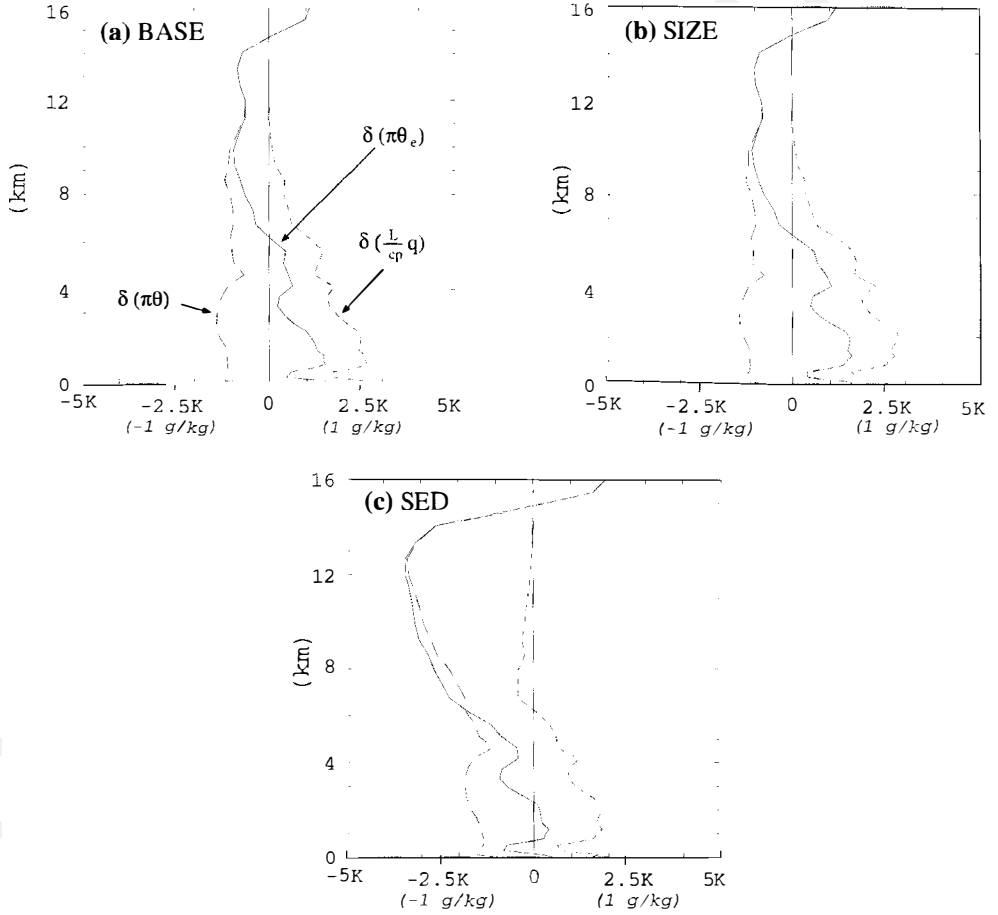
Figure 12. Seven-day-mean difference between simulated and observed temperature, moisture and equivalent potential temperature, for simulations (a) BASE, (b) SIZE and (c) SED: (T^{\text{mod}} - T^{\text{obs}}) (long dashes), \frac{L_v}{c_p}(q_v^{\text{mod}} - q_v^{\text{obs}}) (short dashes), \pi(\theta_e^{\text{mod}} - \theta_e^{\text{obs}}) (solid line). See text for explanation.
