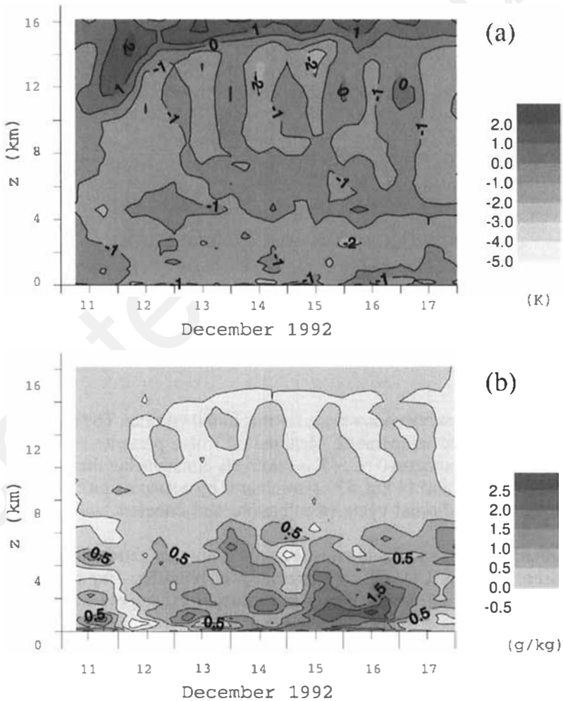
Figure 6. Difference between simulated and observed: (a) temperature T and (b) specific humidity q_v . The contour intervals are 1 K and 0.5 g kg -1 , respectively, and the time average is 6 h.
