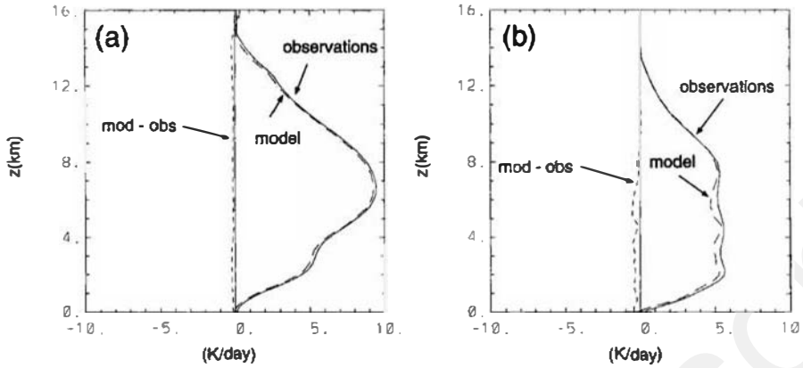
Figure 5. Seven-day-mean profiles of (a) Q_1 and (b) Q_2 (see text), diagnosed from observations (solid line), simulated (short dashes), and the difference 'simulation minus observation' (short dashes).
