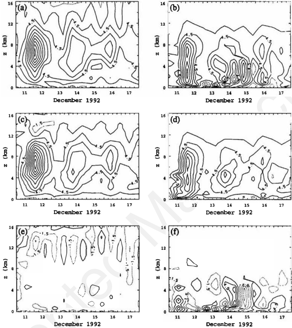
Figure 4. Temporal evolution of (a) the apparent heat source Q_1 and (b) apparent moisture sink Q_2 diagnosed from observations, (c) and (d) simulated Q_1 and Q_2 , and (e) and (f) differences between simulated and observed. The contour interval is 3 \text{ K d}^{-1} starting from the 1.5 isoline (not the zero isoline) and the time average is 6 h.
