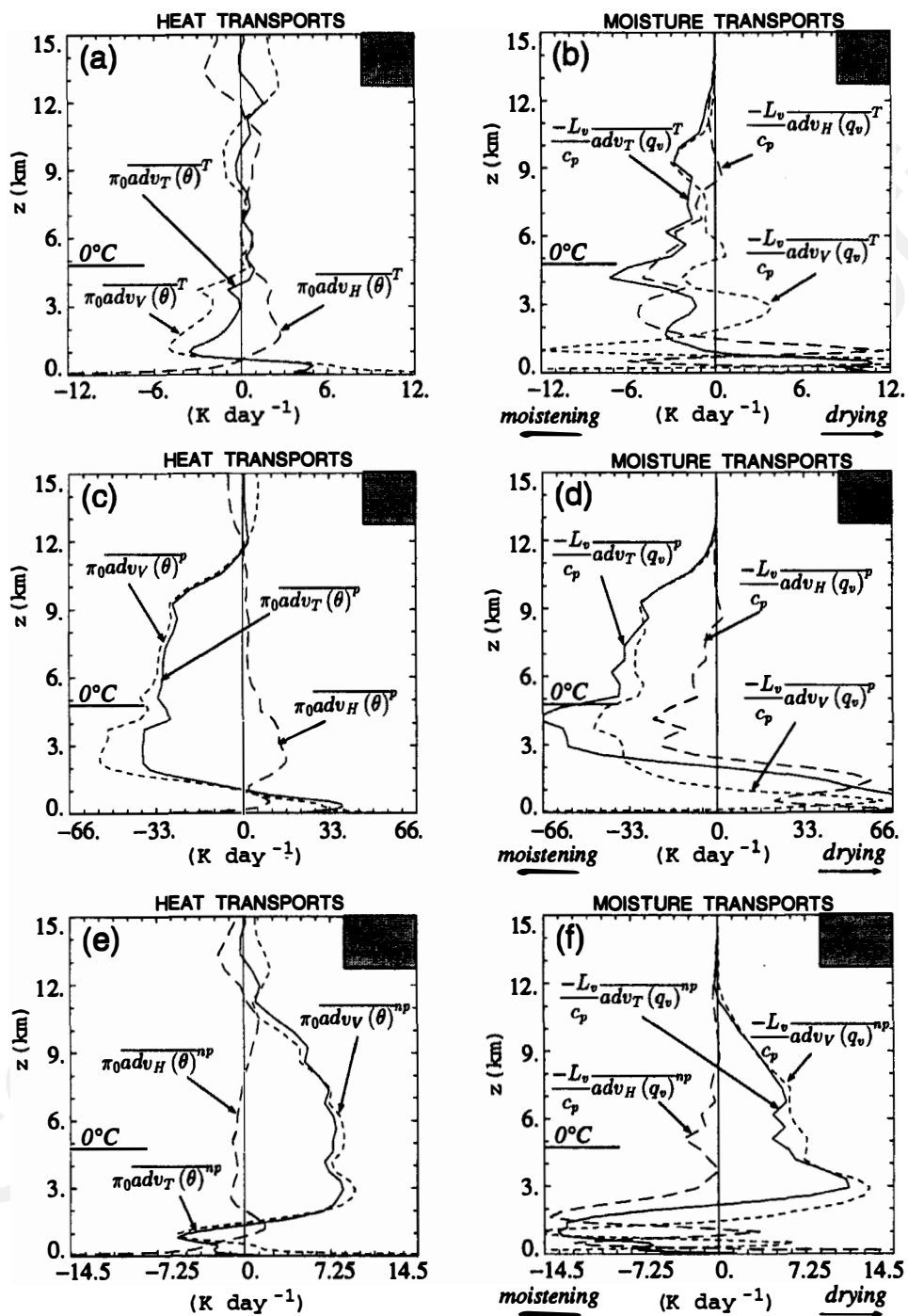
Figure 15. Same as Fig. 14 but for total transports, and their decomposition into horizontal and vertical advectons, with similar horizontal scales.
