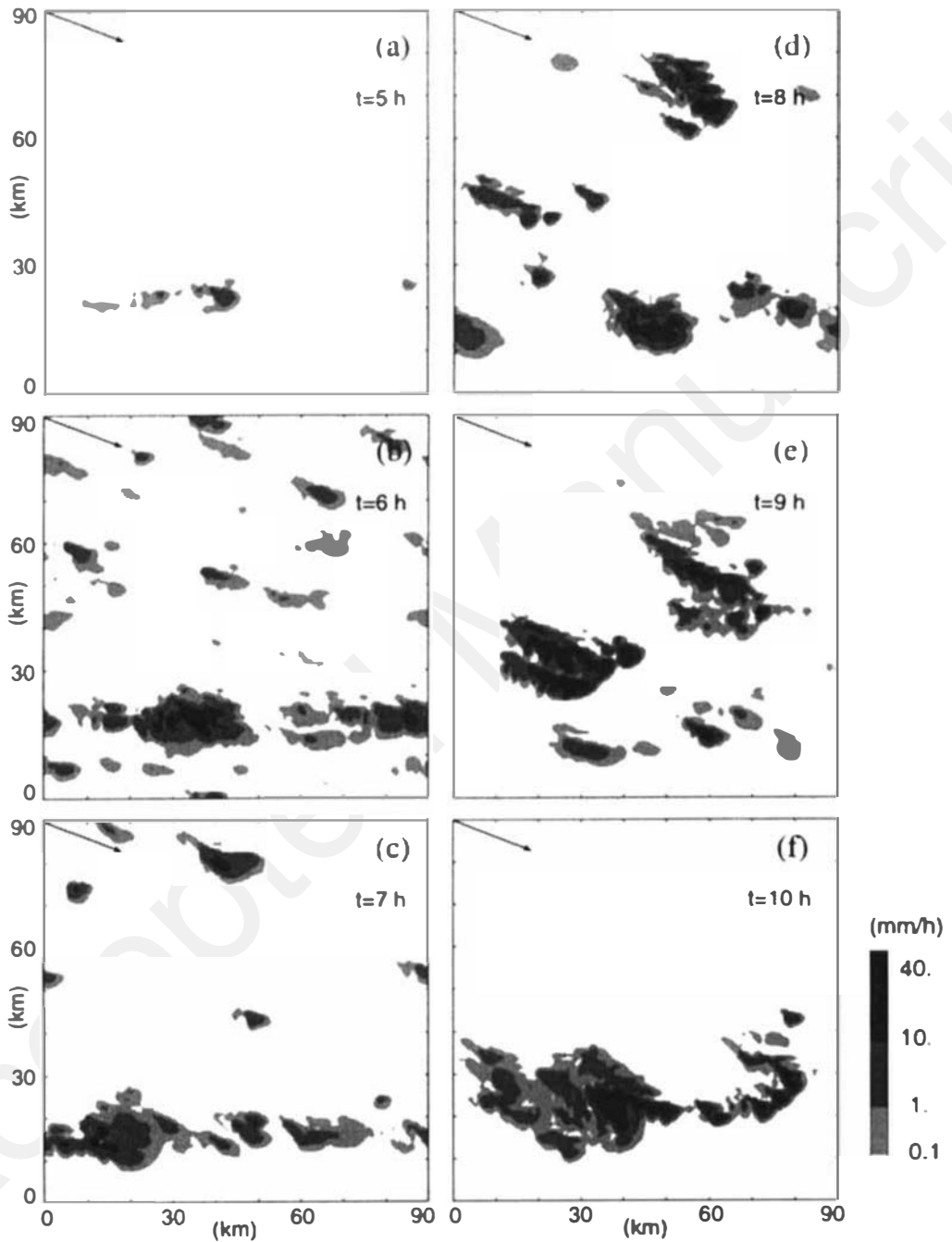
Figure 4. Instantaneous fields of surface precipitation at t = 5 \text{ h} , 6 \text{ h} , 7 \text{ h} , 8 \text{ h} , 9 \text{ h} , and 10 \text{ h} . The arrow shows the horizontal displacement of the area (relative to the surface) in one hour (i.e. between two consecutive pictures), due to a translation of 5 \text{ m s}^{-1} from west to east and 2 \text{ m s}^{-1} from north to south.
