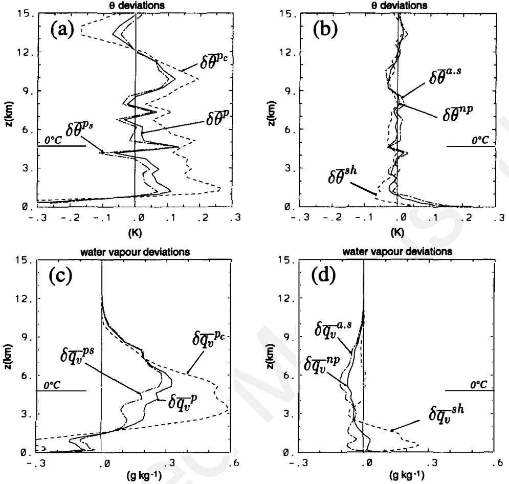
Figure 12. (a) and (b): same as Fig. 9 (a) and (b) but for deviations of potential temperature; (c) and (d): same as (a) and (b) but for deviations of water vapour q_v - \bar{\delta\alpha}^x = \alpha^x - \bar{\alpha}^T .
