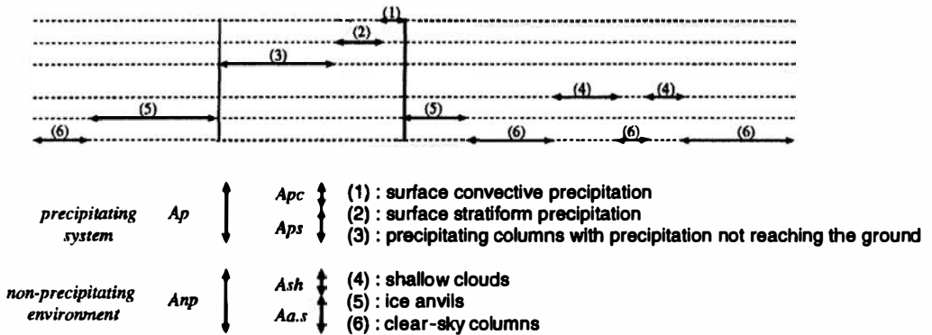
Figure 1. Schematic view of the cloud ensemble and its decomposition.
