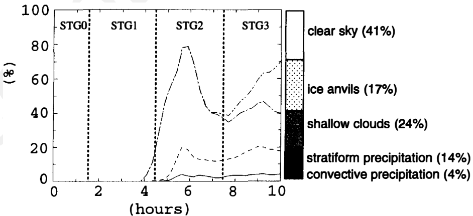
Figure 8. Time history from 0 h to 10 h of area occupancy for: convective precipitation A_{pc} (solid line), the precipitating system A_p (dashed lines), A_p plus shallow-cloud area A_{sh} (dashed-dotted line), A_p plus A_{sh} plus anvil clouds (dashed-dotted-dotted line). Numbers in brackets are the average area occupancies from 8 h to 10 h. See text for further explanation.
