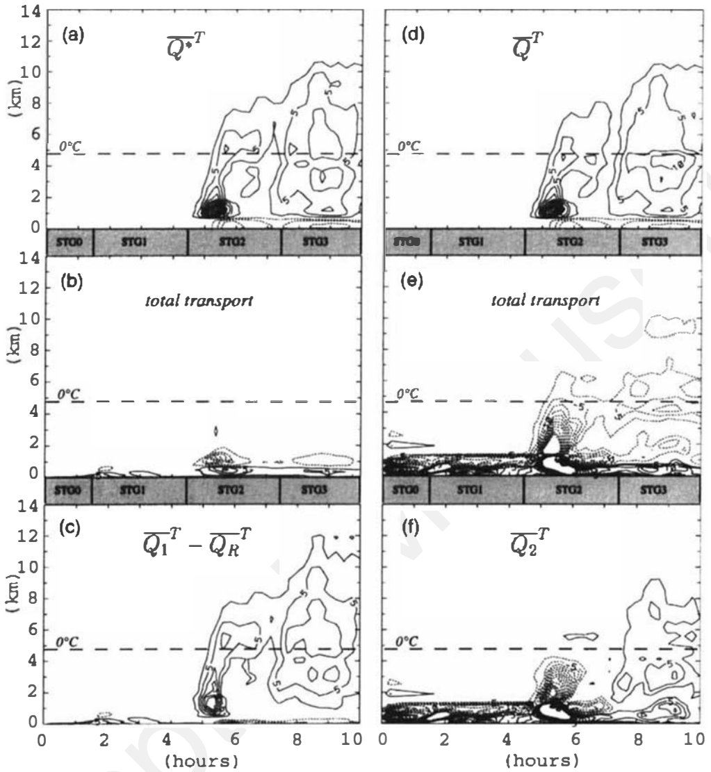
Figure 6. Time evolution averaged at the domain scale A_T , of the heat source budget: (a) total latent-heat release, Q^* , (b) convective transport and (c) convective apparent heat source, Q_1 - Q_R ; and of the moisture sink budget: (d) latent-heat release, Q , (e) convective transport and (f) apparent moisture sink, Q_2 . The time averaging period is \frac{1}{4}h , and the contour interval is 5 \text{ K day}^{-1} . The figures are limited in the vertical to the cloud system depth (14 km). See text for further explanation.
