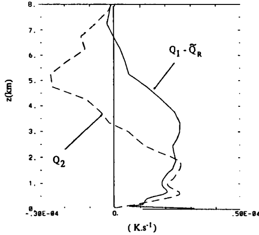
Figure 10. Vertical profiles of Q_1 - \widetilde{Q}_R and Q_2 averaged over the period from 8 h to 48 h for experiment REF.
