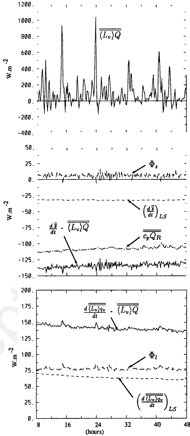
Figure 6. Evolution with time over the period 8 h to 48 h for experiment REF of: (a) \overline{\overline{(L_v)Q}} ; and, of the other terms of the budgets, of: (b) \bar{s} ; (c) \overline{\overline{(L_v)q_v}} , with the time average T taken equal to 10 min (see text for definition).
