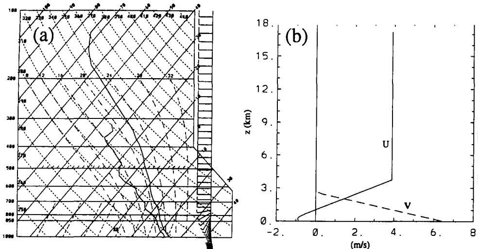
Figure 2. Initial vertical profiles: (a) skew- T log- P diagram; (b) wind components ( \text{m s}^{-1} ).
