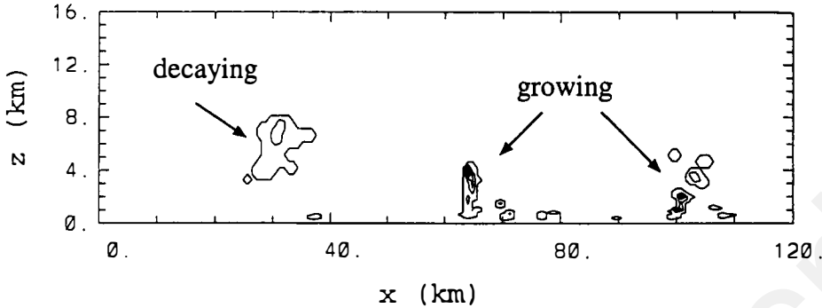
Figure 4. Vertical cross-sections of cloud field at 25 h 30 min for experiment REF.
