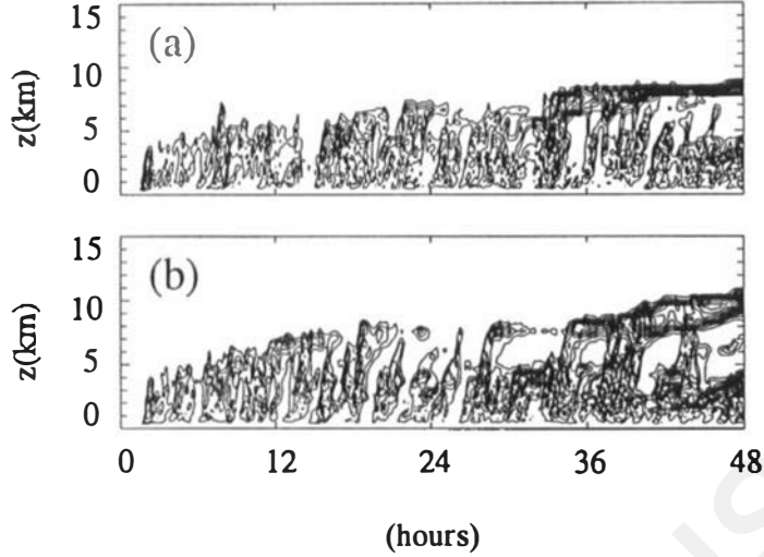
Figure 16. Same as for Fig. 5(a), but for experiments: (a) HIGHLS 1; (b) HIGHLS 2. Values of \tilde{q}_c are averaged over 10 min, with a contour interval of 10^{-5} . The lower contour is 10^{-5} ; the higher contours are 13 \times 10^{-5} for HIGHLS 1 and 17 \times 10^{-5} for HIGHLS 2.
