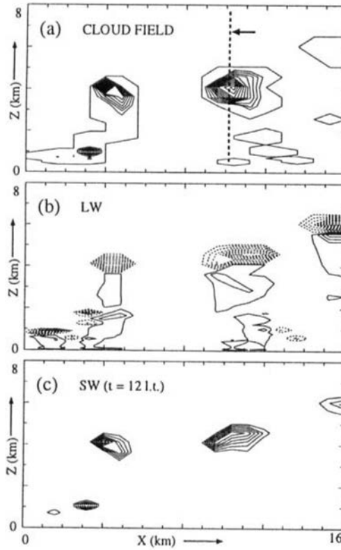
Figure A.1. Vertical cross-section in part of the domain of: (a) q_c at 1.5 \times 10^{-4} \text{ kg kg}^{-1} intervals, lower and higher contours are 0 \text{ kg kg}^{-1} and 2.1 \times 10^{-3} \text{ kg kg}^{-1} , respectively; (b) longwave radiative flux divergence at 5 \text{ K d}^{-1} intervals, lower and higher contours are -50 \text{ K d}^{-1} and 15 \text{ K d}^{-1} , respectively; (c) shortwave radiative flux divergence at 5 \text{ K d}^{-1} intervals, lower and higher contours are 0 \text{ K d}^{-1} and 40 \text{ K d}^{-1} , respectively.
