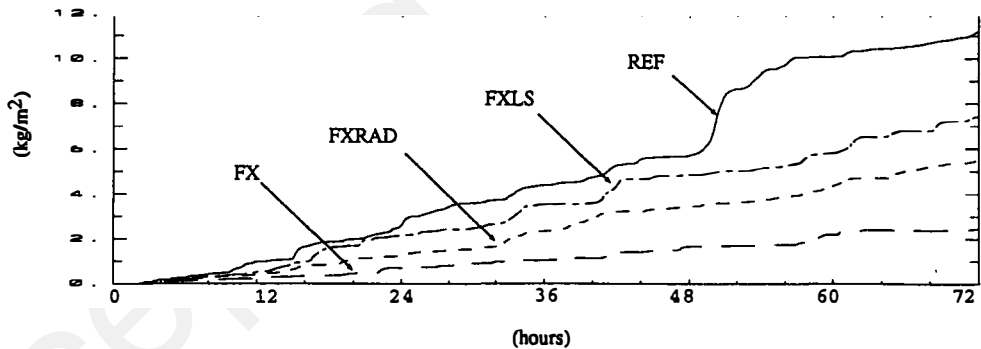
Figure 12. Cumulative precipitation for experiments REF, FX, FXRAD and FXLS.
