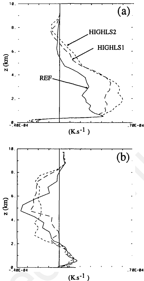
Figure 19. Same as for Fig. 14, but averaged over the period 8 h to 32 h and for experiments HIGHLS 1 and HIGHLS 2.
