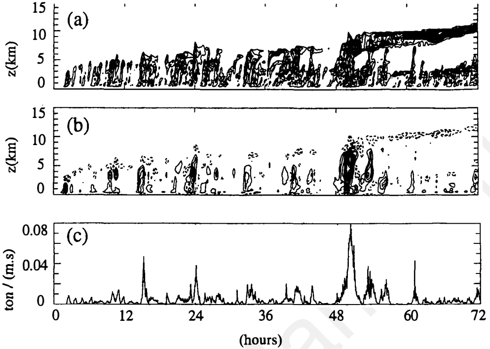
Figure 5. Evolution with time for experiment REF of: (a) average cloud water content \tilde{q}_c (kg kg -1 ); (b) net condensation rate ((L_v)/c_p)\bar{Q} , (K s -1 ); (c) precipitation rate. Values of \tilde{q}_c are averaged over 10 min; the contour interval is 10^{-5} (lower and higher contours are 10^{-5} and 15 \times 10^{-5} , respectively). Values of ((L_v)/c_p)\bar{Q} are averaged over 30 min; the contour interval is 5 \times 10^{-5} for positive values (continuous lines; lower and higher contours are 5 \times 10^{-5} and 5 \times 10^{-4} , respectively) and 2.5 \times 10^{-5} for negative values (dotted lines; lower and higher contours are -1.25 \times 10^{-4} and -2.5 \times 10^{-5} , respectively).
