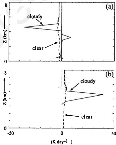
Figure A.2. Vertical profiles of the divergence of: (a) longwave and (b) shortwave radiative fluxes in clear and cloudy conditions for the vertical cross-section indicated in Fig. A.1.
