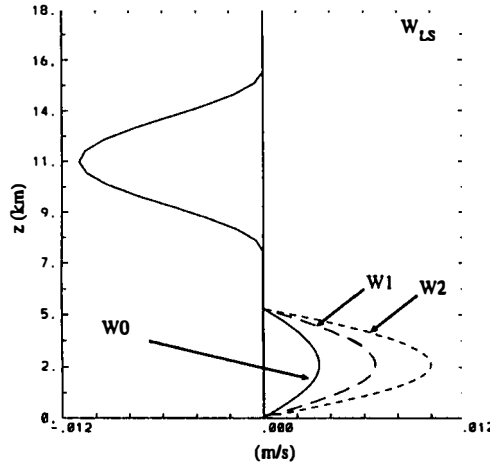
Figure 3. Large-scale ascent profiles.
