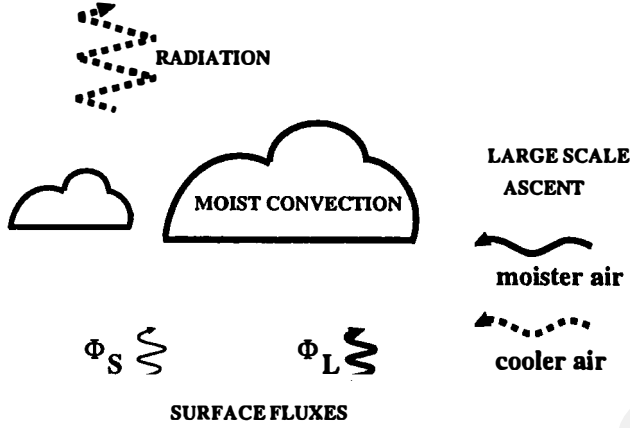
Figure 1. Schematic diagram showing the four interacting processes.
