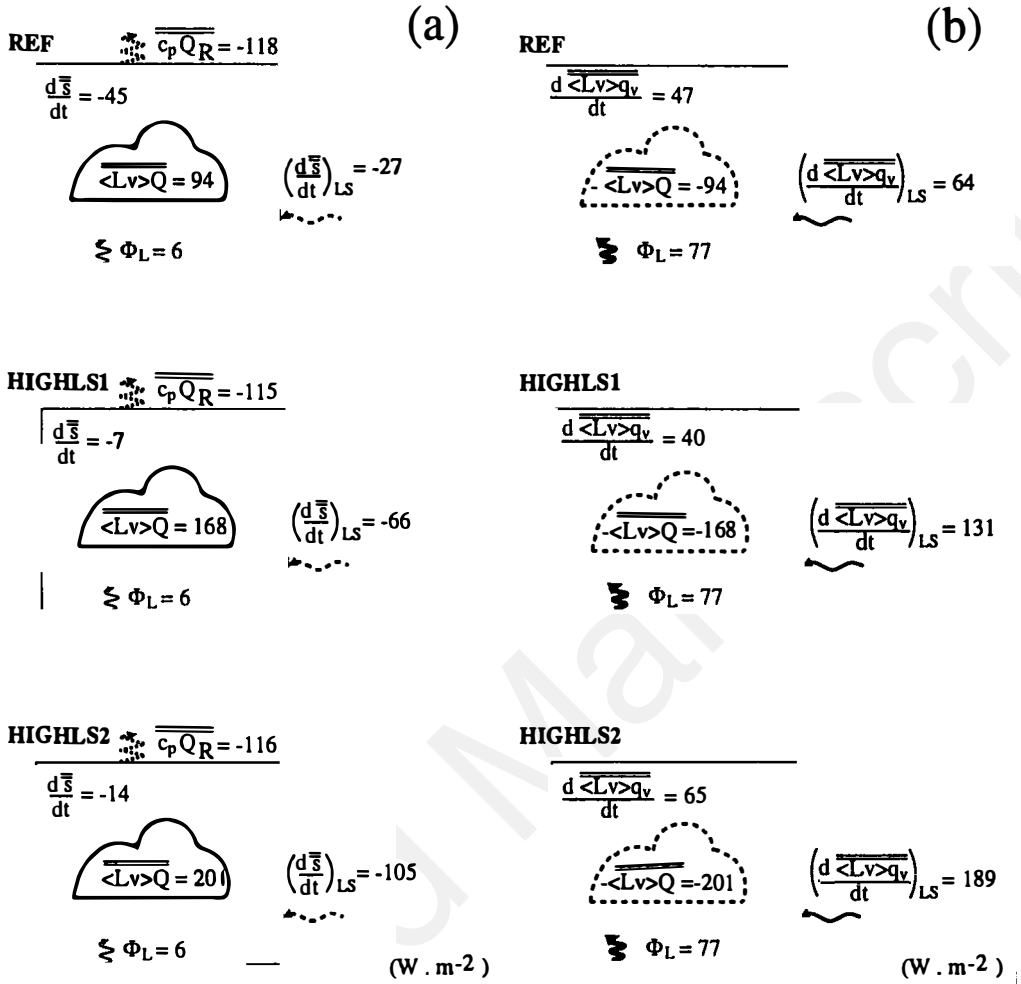
Figure 18. OD budgets of: (a) \bar{s} ; (b) \langle Lv \rangle q_v , averaged over the period 8 h to 32 h for experiments HIGHLS 1 and HIGHLS 2.
