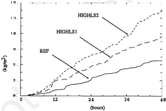
Figure 17. Same as for Fig. 12, but for experiments REF, HIGHLS 1 and HIGHLS 2.
