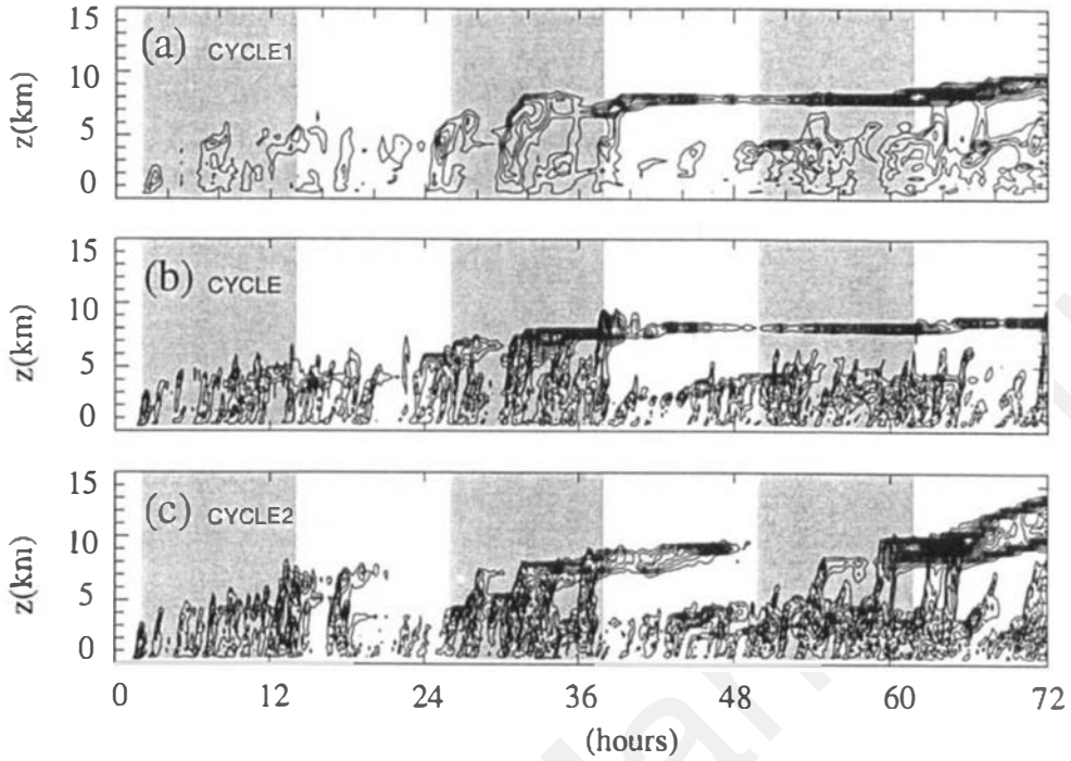
Figure 20. Same as for Fig. 5(a) but for experiments: (a) CYCLE 1; (B) CYCLE; (c) CYCLE 2 (contour interval of 10^{-5} ); the lower contour is 10^{-5} and the higher contours are 15 \times 10^{-5} for CYCLE 1, 14 \times 10^{-5} for CYCLE and 25 \times 10^{-5} for CYCLE 2. Grey corresponds to night-time.
