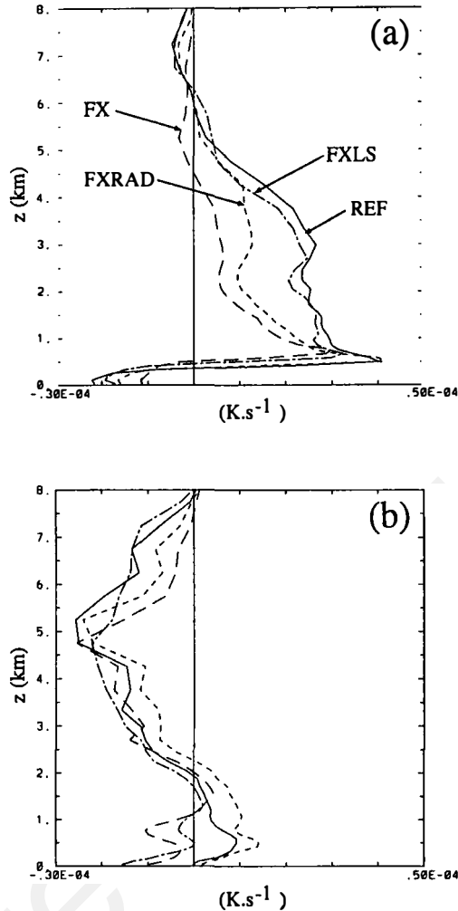
Figure 14. Vertical budgets averaged over the period 8 h to 48 h for experiments REF, FX, FXRAD and FXLS of: (a) \langle(L_v)/c_p\rangle\dot{Q} ; (b) -\langle(L_v)/c_p\rangle\partial q_v/\partial t .
