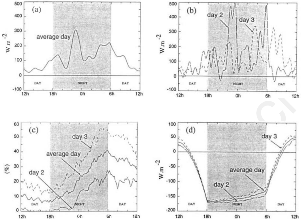
Figure 22. Diurnal evolution for experiments CYCLE 1, CYCLE and CYCLE 2 of \overline{\langle L_v \rangle Q} (low-pass filter of 80 min): (a) averaged over the two last days; (b) over the 2nd and 3rd days, and of (c) the maximum cloud fraction above 7 km; (d) the net radiative heating over the layer 0 to 8 km for the same periods.
