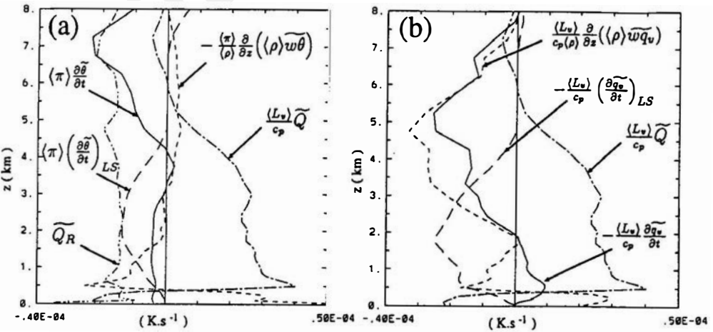
Figure 9. Vertical budgets averaged over the period from 8 h to 48 h for experiment REF of (a) \langle \pi \rangle \tilde{\theta} ; (b) -(L_v/c_p) \tilde{q}_v .
