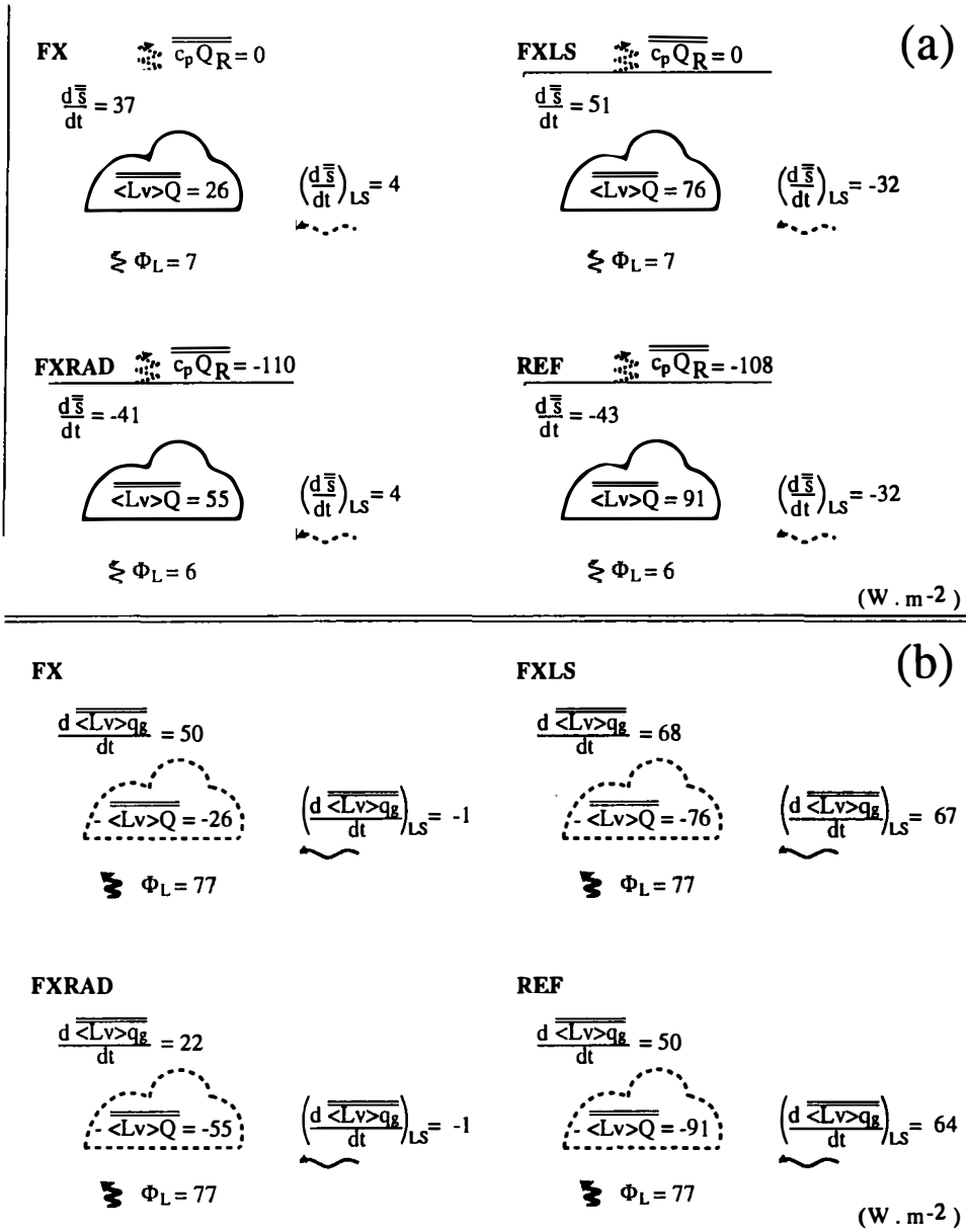
Figure 13. Budgets averaged over the period 8 h to 48 h for experiment REF, FX, FXRAD and FXLS of: (a) \overline{s} ; (b) \overline{\langle Lv \rangle q_v} .
