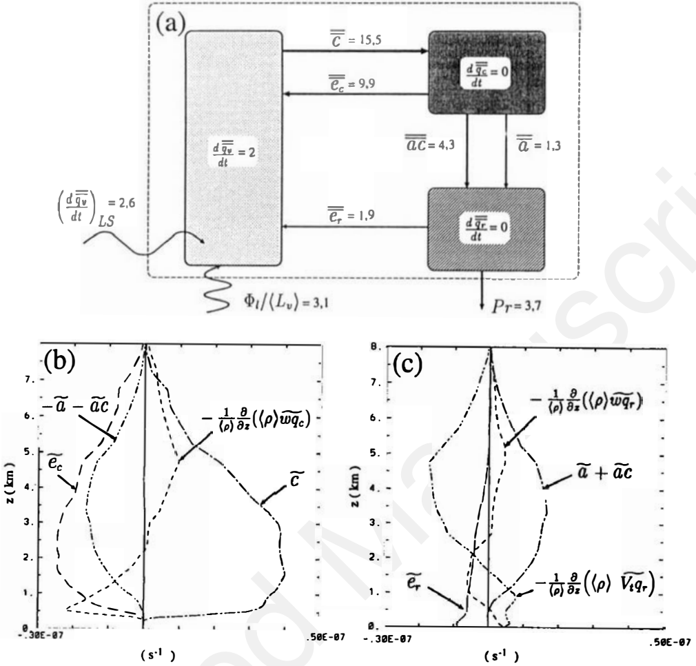
Figure 8. Water budgets averaged over the period from 8 h to 48 h for experiment REF: (a) the OD water-cycle budget, and the 1D budgets of (b) \bar{q}_c and (c) \bar{q}_r .
