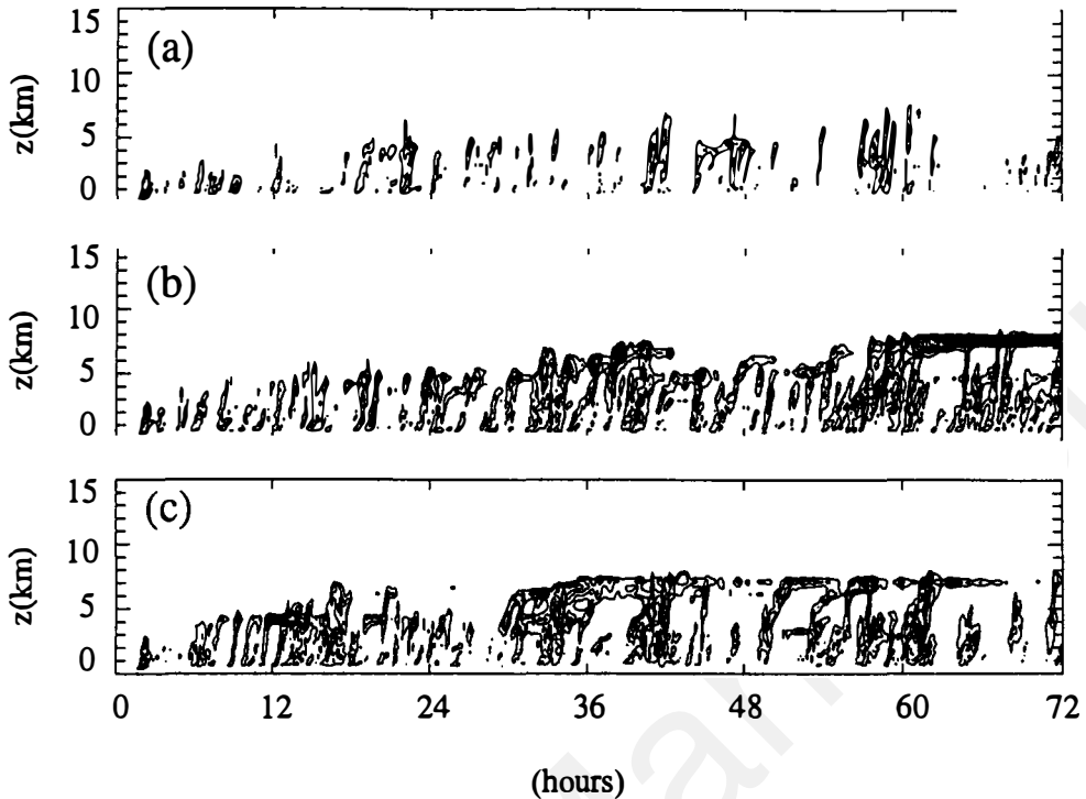
Figure 11. Same as Fig. 5(a), but for experiments (a) FX; (b) FXRAD; (c) FXLS. Values of \tilde{q}_c are averaged over 10 min, contour interval 10^{-5} . The lower contour is 10^{-5} and the higher contours are 4 \times 10^{-5} for FX, 11 \times 10^{-5} for FXRAD and 7 \times 10^{-5} for FXLS.
