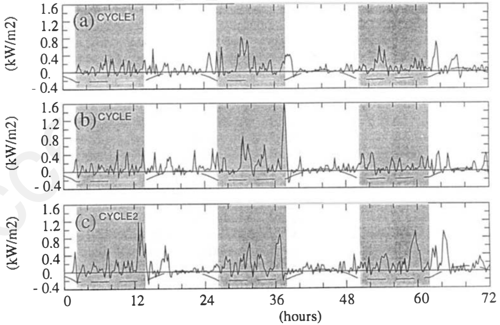
Figure 21. Evolution with time of \overline{\overline{(L_v)Q}} and \overline{\overline{c_p Q_R}} for experiments (a) CYCLE 1; (b) CYCLE; (c) CYCLE 2.
