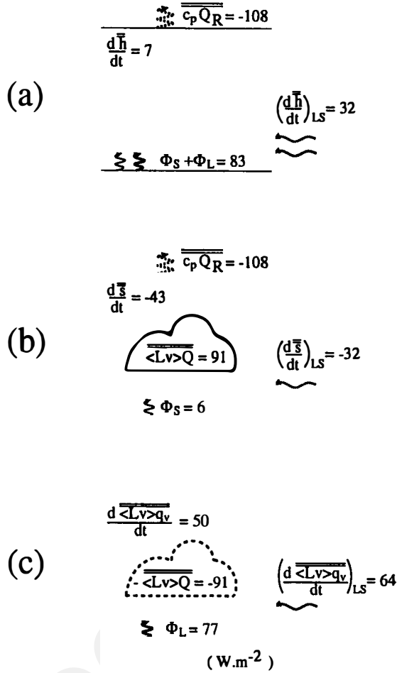
Figure 7. OD budgets averaged over the T period from 8 h to 48 h for experiment REF of: (a) \bar{h} ; (b) \bar{s} ; (c) \langle L_v \rangle q_v , (W m -2 , as for all following OD budgets).
