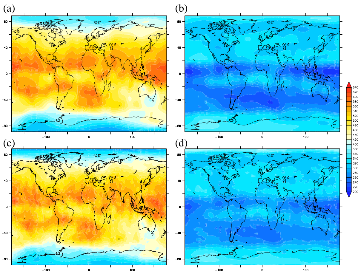
Figure 7. Representation of the raw length-scale estimation over the last twenty days of July 2003 at 10hPa: zonal (a) and meridional (b) length-scale. These field are used to approximate the diffusion coefficients associated to such a heterogeneity. The zonal (c) and meridional (d) length-scale of the resulted formulation are diagnosed using a randomization method with 6400 samples.
