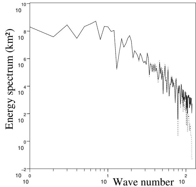
Figure 3. Energy spectrum of initial length-scale field L_{th} (solid line) compared to the diagnosed length-scale field L_{diag} of modelled covariance matrix with the diffusion operator (dotted line).
