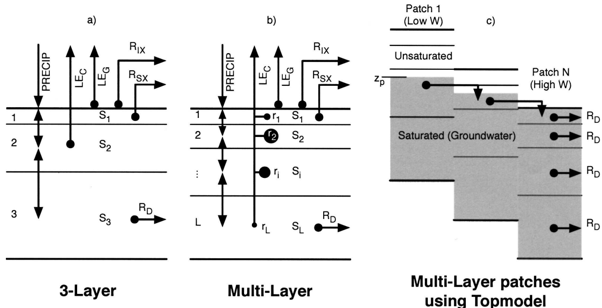
FIG. 2. Soil moisture schemes used in this study: (a) three-layer (3L), (b) multilayer (ML), and (c) multilayer-Topmodel (MLTOP).
