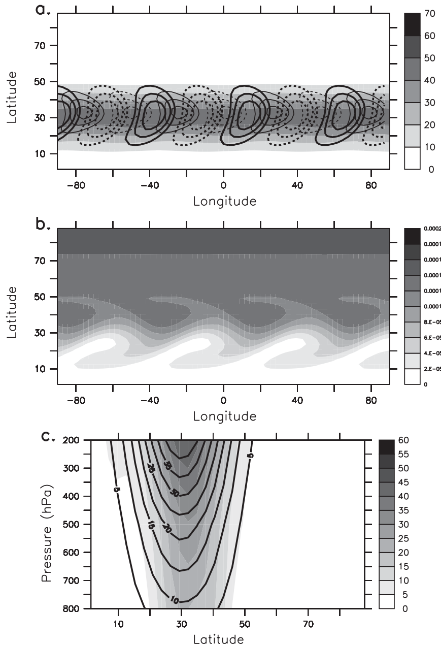
FIG. 5. As in the left column of Fig. 4, but for a 30° jet.
