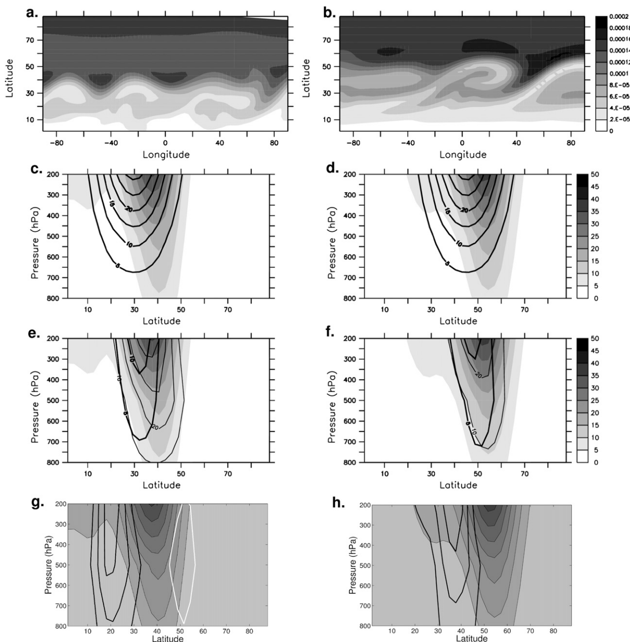
FIG. 14. Comparison between two simulations of the QG model whose restoration-baroclinicity fields are centered at (left) 30°N and (right) 45°N. (a),(b) Snapshot of absolute vorticity at 200 hPa (interval: 2 \times 10^{-5} \text{ s}^{-1} ). (c),(d) Meridional cross sections of time-averaged zonally averaged zonal winds with (shading) and without (black contours) an initial perturbation (interval: 5 \text{ m s}^{-1} ). (e),(f) High-frequency kinetic energy (light solid contours; interval: 10 \text{ m}^2 \text{ s}^{-2} ) and momentum fluxes (thick black contours; solid and dashed lines indicate positive and negative values, respectively; interval: 5 \text{ m}^2 \text{ s}^{-2} ). (g),(h) Zonal average of CWB and AWB frequencies, \gamma_c (white contours; interval: 0.1) and \gamma_a (heavy black contours; interval: 0.1). Shaded areas in (e),(g) and (f),(h) are the same as in (c) and (d), respectively.
