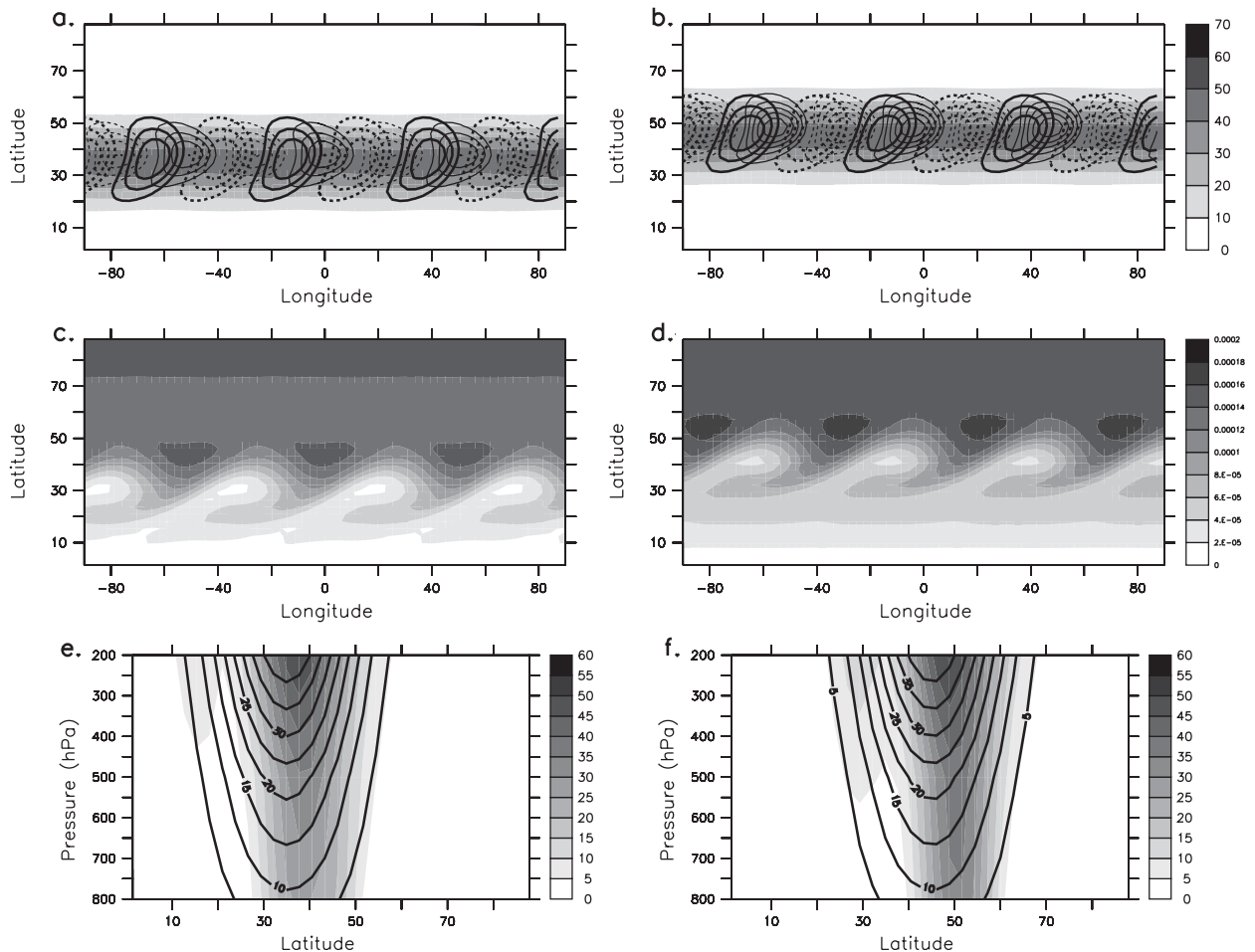
FIG. 4. Normal-mode structure and evolution using the QG model for a wavenumber-7 disturbance embedded in a (left) 35° and (right) 45° jet. (a),(b) Basic-state zonal winds (shading; interval: 10 \text{ m s}^{-1} ) and normal-mode meridional velocities at 200 hPa (heavy contours) and 800 hPa (light contours) normalized by the maximum at the upper level (interval: 0.2). (c),(d) Absolute vorticity after 6 days (interval: 2 \times 10^{-5} \text{ s}^{-1} ). (e),(f) Meridional cross sections of zonally averaged zonal winds at the initial time (black contours) and after 10 days (shading; interval: 5 \text{ m s}^{-1} ).
