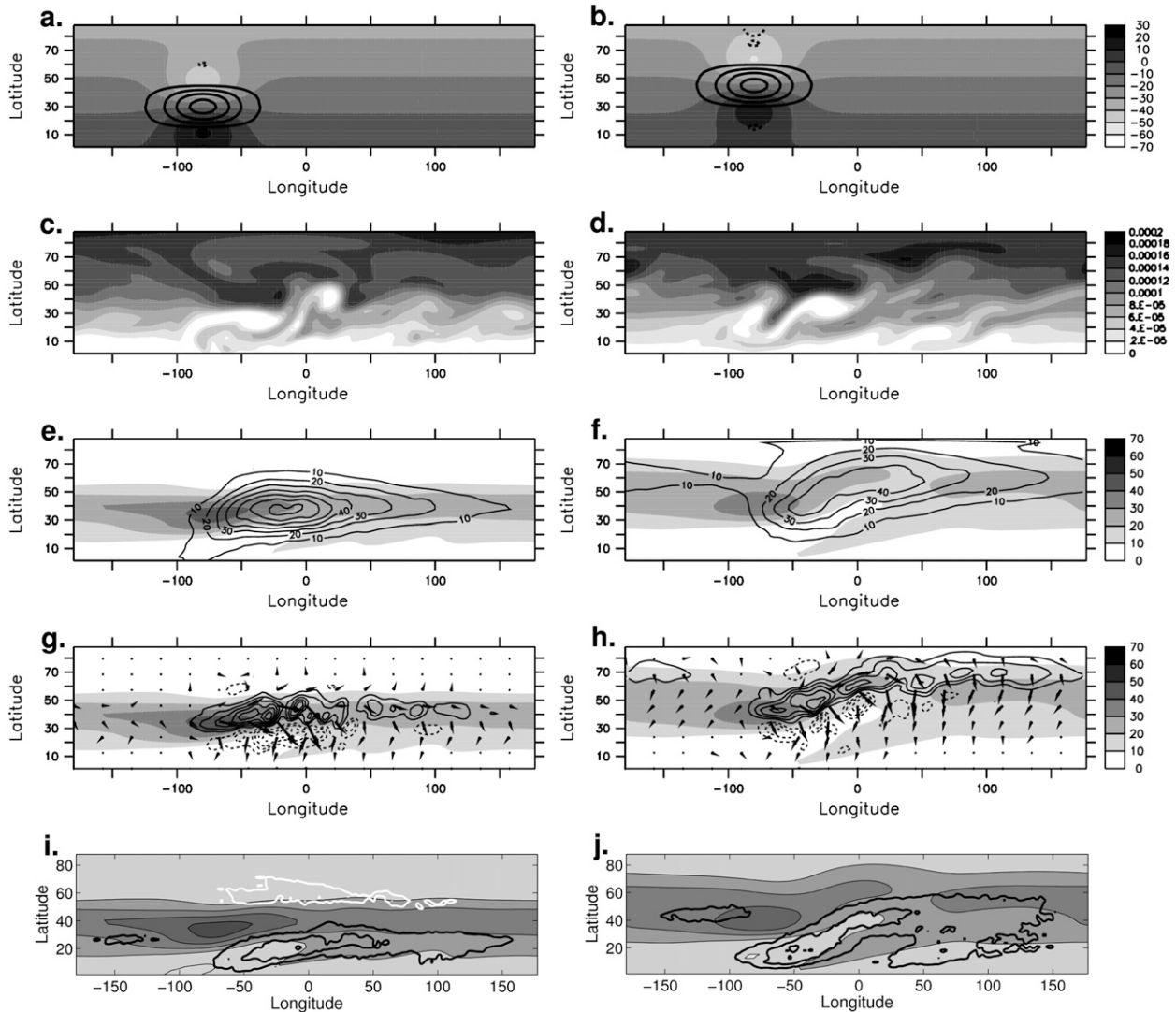
FIG. 18. Comparison between two Z-shaped simulations of the QG model whose restoration-baroclinicity fields are centered at (left) 30^\circ\text{N} , 80^\circ\text{W} and (right) 45^\circ\text{N} , 80^\circ\text{W} . (a),(b) Restoration temperature at 650 hPa (interval: 10^\circ\text{C} ) and the related baroclinicity ( R_{02}^{-1}(\partial\bar{\psi}_2/\partial y - \partial\bar{\psi}_3/\partial y) ; interval: 2 \times 10^{-5} \text{ s}^{-1} ; solid and dashed lines for positive and negative values). (c),(d) Snapshot of absolute vorticity at 200 hPa (interval: 2 \times 10^{-5} \text{ s}^{-1} ). (e),(f) Time-mean zonal wind (shadings; interval: 10 \text{ m s}^{-1} ) and high-frequency kinetic energy (black contours; interval: 10 \text{ m}^2 \text{ s}^{-2} ) at 200 hPa. (g),(h) \mathbf{E} vector and (1/\cos\phi)\nabla \cdot (\mathbf{E}\cos\phi) (black contours; interval: 5 \times 10^{-6} \text{ m s}^{-2} ) at 200 hPa. (i),(j) CWB and AWB frequencies \gamma_c (white contours; interval: 0.1) and \gamma_a (heavy black contours; interval: 0.1) at 200 hPa. Shadings in (g),(i) and (h),(j) are the same as in (e) and (f), respectively.
