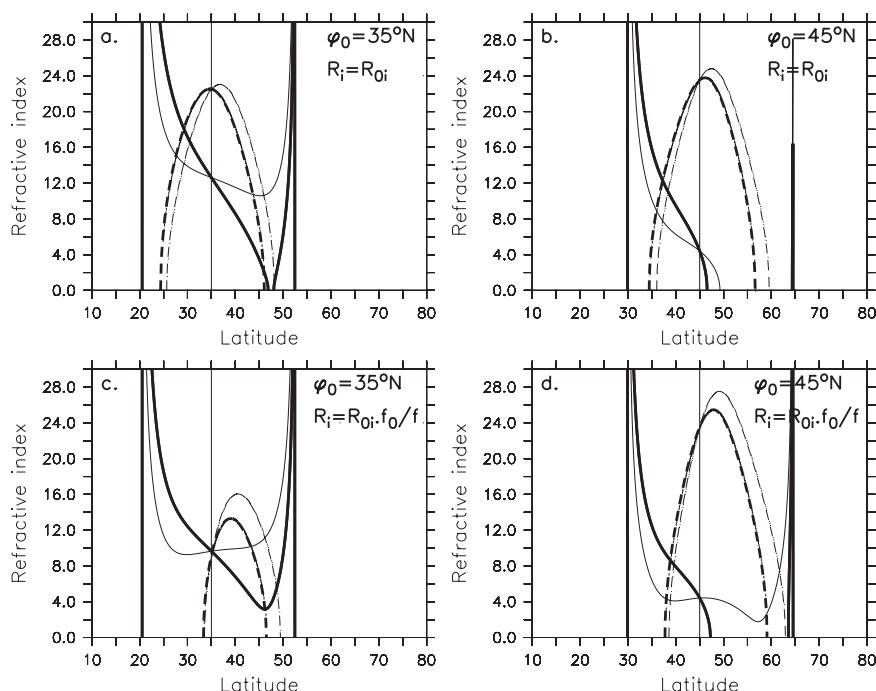
FIG. 3. Refractive index defined as \ln|\text{sign}(n^2)| (nondimensional values) at 200 hPa (thick solid lines) and at 800 hPa (thick dashed lines) for (a) R_i = R_{0i} , \varphi_0 = 35^\circ\text{N} , (b) R_i = R_{0i} , \varphi_0 = 45^\circ\text{N} , (c) R_i = R_{0i}f_0/f , \varphi_0 = 35^\circ\text{N} , and (d) R_i = R_{0i}f_0/f , \varphi_0 = 45^\circ\text{N} . The thin lines correspond to the refractive index when \varphi is replaced by \varphi_0 in all terms of Eq. (5) apart from the first term, where the full variations of \varphi are kept. All n^2 are computed for m = 7 , c = 3 \times 10^{-6} \text{ s}^{-1} , H = 8000 \text{ m} , and N = 0.01 \text{ s}^{-1} . Other values are given in the text.
