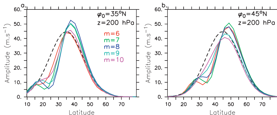
FIG. 7. Zonally averaged zonal winds at 200 hPa after 10 days as function of zonal wavenumber using the OG model for the (a) 35° and (b) 45° jets. Zonal winds corresponding to wavenumbers 6, 7, 8, 9, and 10 are respectively represented by the lines in red, green, blue, light blue, and magenta. The zonal wind at the initial time is represented by the black dashed line.
