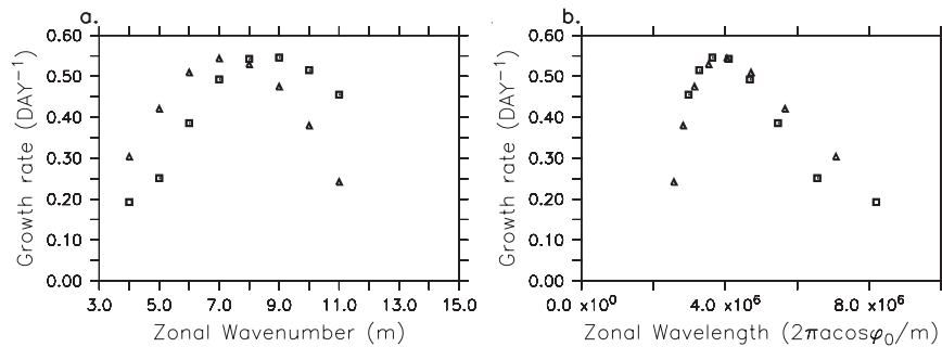
FIG. 6. Normal-mode growth rates using the OG model as function of (a) zonal wavenumber and (b) zonal wavelength for the 35° (squares) and 45° jet (triangle).
