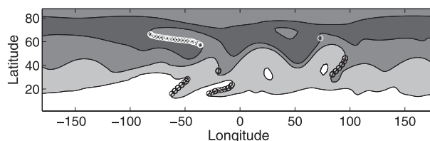
FIG. C1. Illustration of the wave-breaking detection method. The 4, 10 , and 14 \times 10^{-5} \text{ s}^{-1} contours of absolute vorticity are represented by solid lines and shaded areas (same case as in Fig. 19d). All points belonging to a segment along a circumpolar contour detected as CWB and AWB regions are shown by open circles (white for CWB and black for AWB). See more details in the text.
