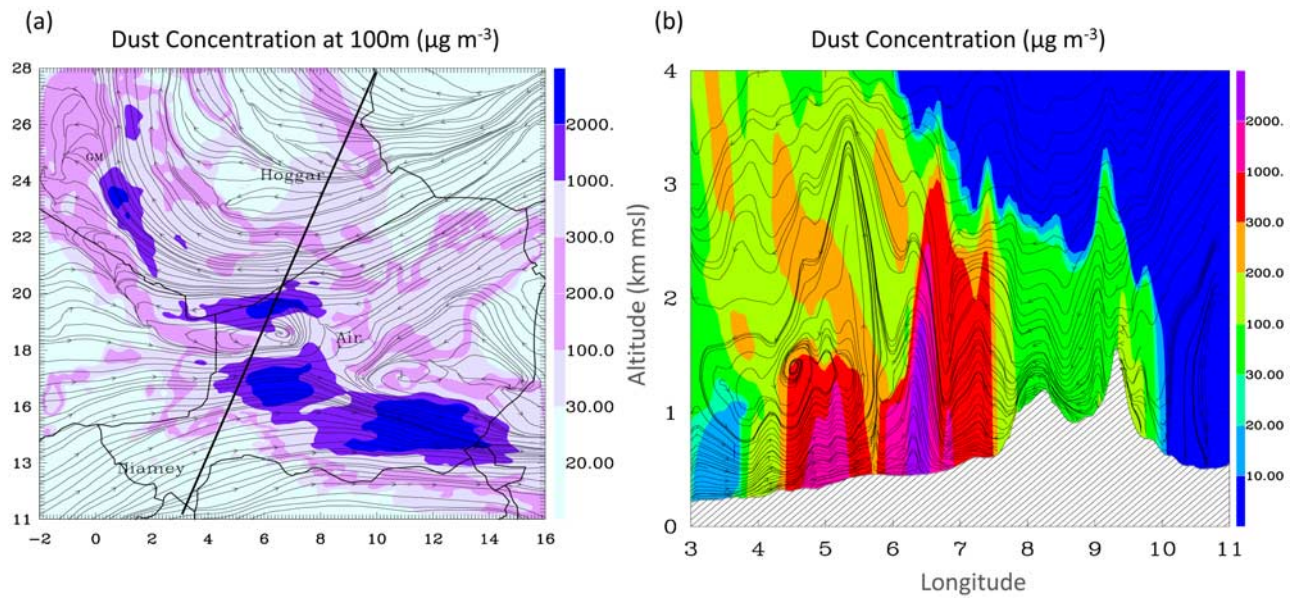
Figure 8. (a) Dust concentrations (color) derived from MesoNH simulation and streamlines at 100 m agl at 1100 UTC on 7 July. (b) Vertical cross section through the cyclone along the black line shown in Figure 8a of dust concentrations (color) and streamlines at 1100 UTC on 7 July.
