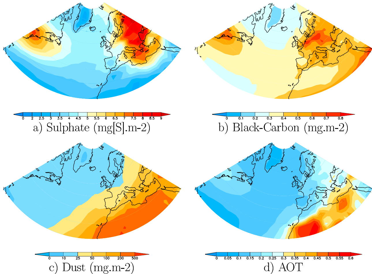
Figure 2. Sulfate ( \text{mg[S]} \text{ m}^{-2} ), black carbon ( \text{mg m}^{-2} ), dust ( \text{mg m}^{-2} ), and aerosol optical thickness (AOT) winter average from 2000 to 2005 simulated by MOCAGE.
