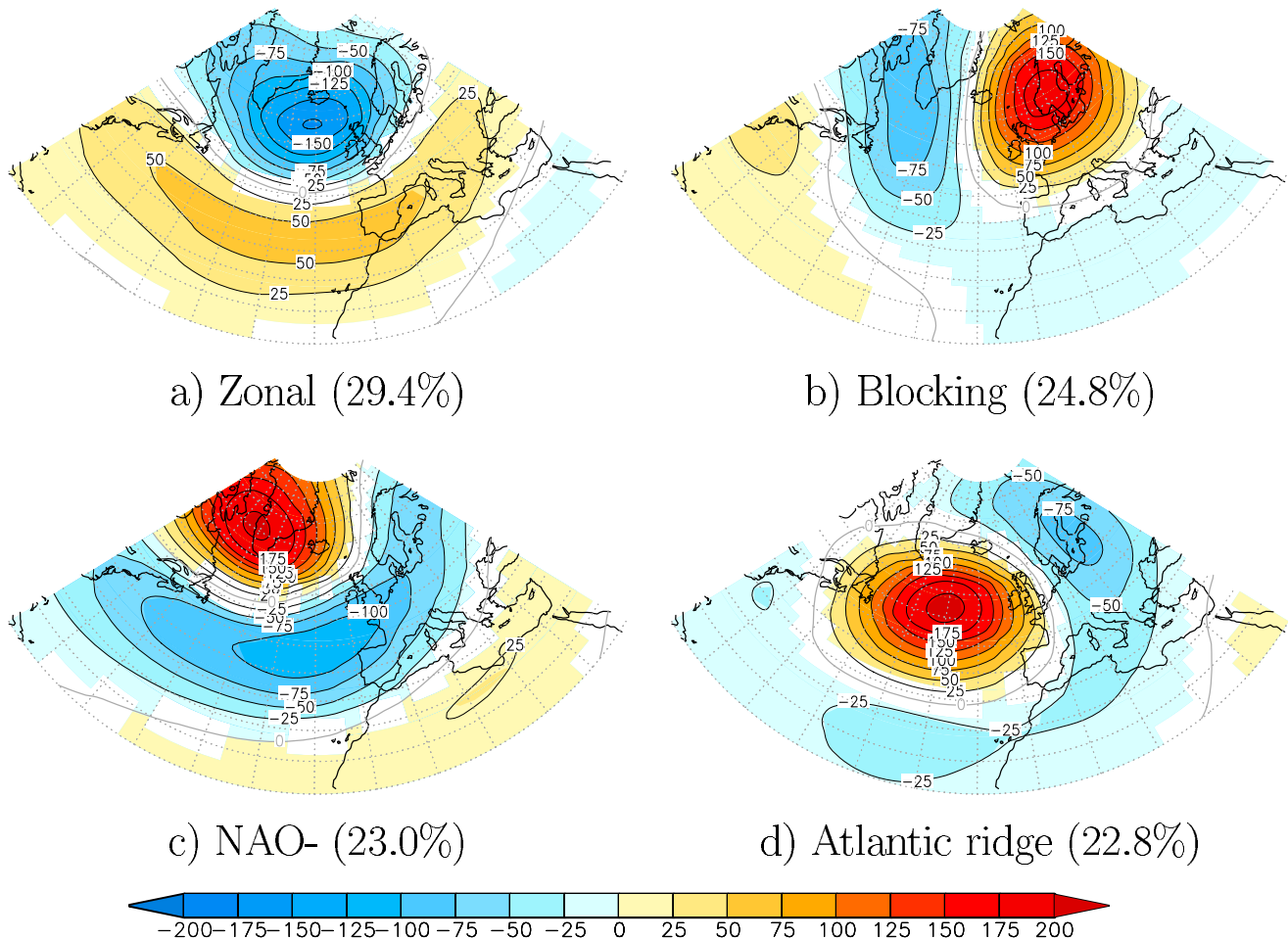
Figure 3. Composites of the anomalies of ERA40 500 hPa geopotential height anomalies (m) corresponding to the four North Atlantic weather regimes in winter (December–February): (a) zonal; (b) blocking; (c) NAO–; (d) Atlantic ridge. Weather regime frequencies are in parentheses. The contour interval is 25 m; 95% significant values are shown in color.
