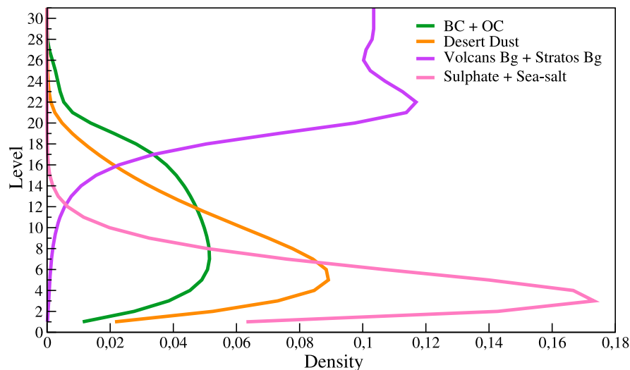
Figure 10. Aerosol profiles prescribed in the 31-level ARPEGE-Climat model.
