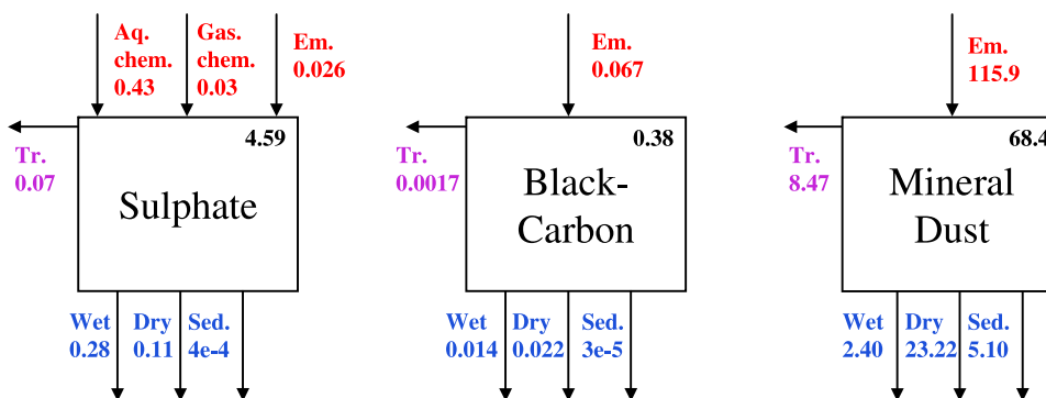
Figure 1. Sulfate, black carbon, and mineral dust budget over the North Atlantic region (20°N–80°N, 80°W–40°E) in winter (December–February) from 2000 to 2005. Burdens (top right corner of the square) are given in mg[S] m -2 for sulfate and in mg m -2 for the other aerosols. Fluxes are given in mg[S] m -2 d -1 for sulfate and in mg m -2 d -1 for the other aerosols. Tr., transport outside of the domain; Wet, wet deposition; Dry, dry deposition; Sed., sedimentation; Aq. chem., aqueous chemistry; Gas. chem., gaseous chemistry; Em., emissions.
