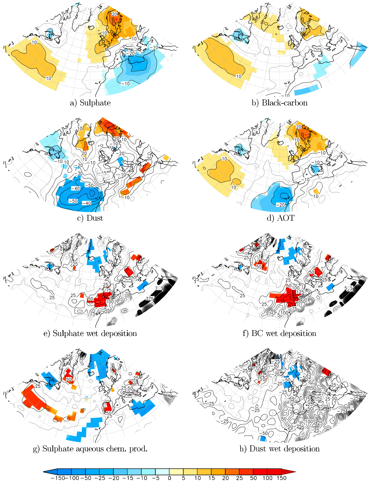
Figure 8. The 2000–2005 DJF NAO– regime anomalies (in percentage) of sulfate burden, black carbon (BC) burden, dust burden, aerosol optical thickness (AOT), sulfate wet deposition, BC wet deposition, sulfate aqueous chemical production, and dust wet deposition over the North Atlantic region; 95% significant values are drawn in color.
