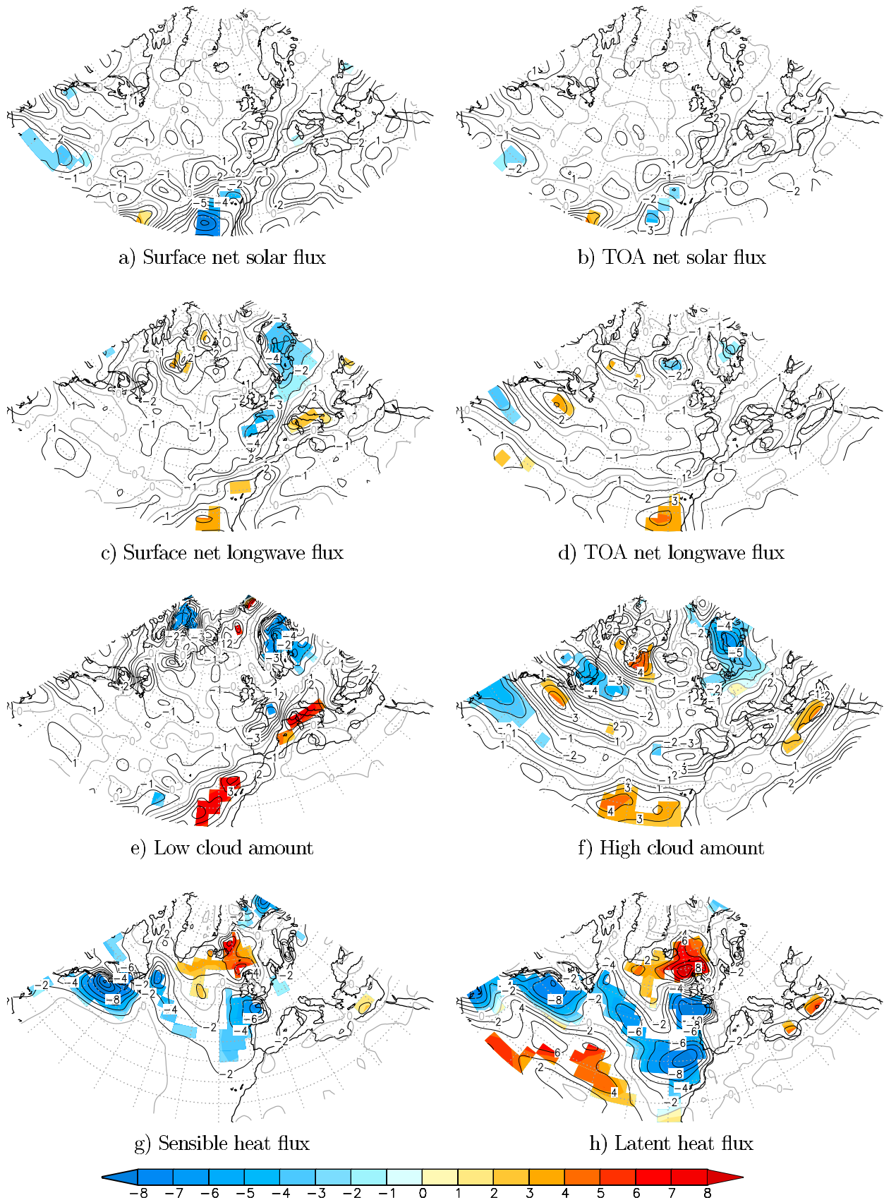
Figure 11. Differences in heat fluxes (in \text{W m}^{-2} ) and low and high cloud amounts (in percentage) (AER-ZO – CTL) during the NAO– regime (see text for description). Positive fluxes are directed downward.
