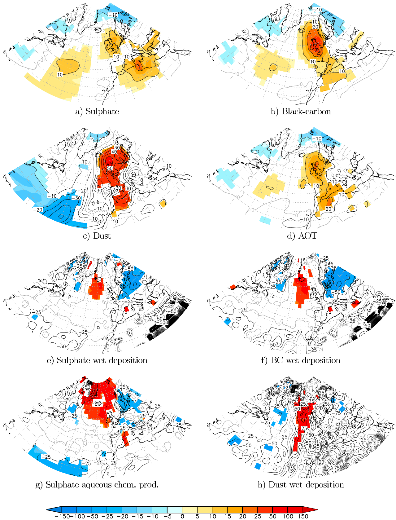
Figure 7. The 2000–2005 DJF blocking regime anomalies (in percentage) of sulfate burden, black carbon (BC) burden, dust burden, aerosol optical thickness (AOT), sulfate wet deposition, BC wet deposition, sulfate aqueous chemical production, and dust wet deposition over the North Atlantic region; 95% significant values are shown in color.
