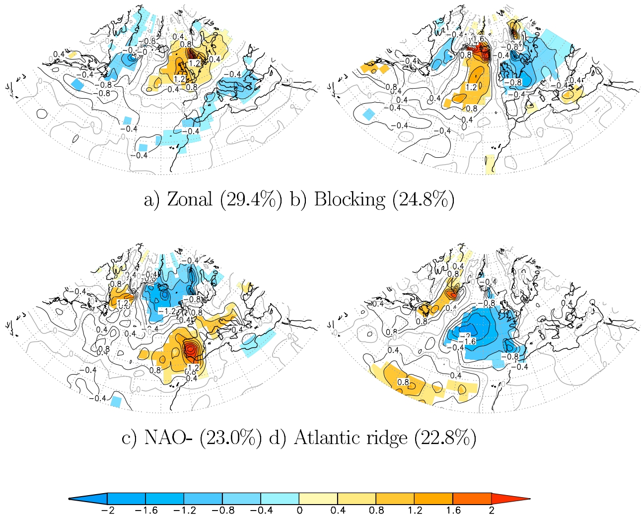
Figure 4. Composites of 2000–2005 ECMWF/MOCAGE (see text for description) liquid precipitation anomalies ( \text{mm d}^{-1} ) during the days for which the atmosphere is classified as (a) zonal, (b) blocking, (c) NAO-, or (d) Atlantic ridge,. The contour interval is 0.4; 95% significant values are shown in color.
