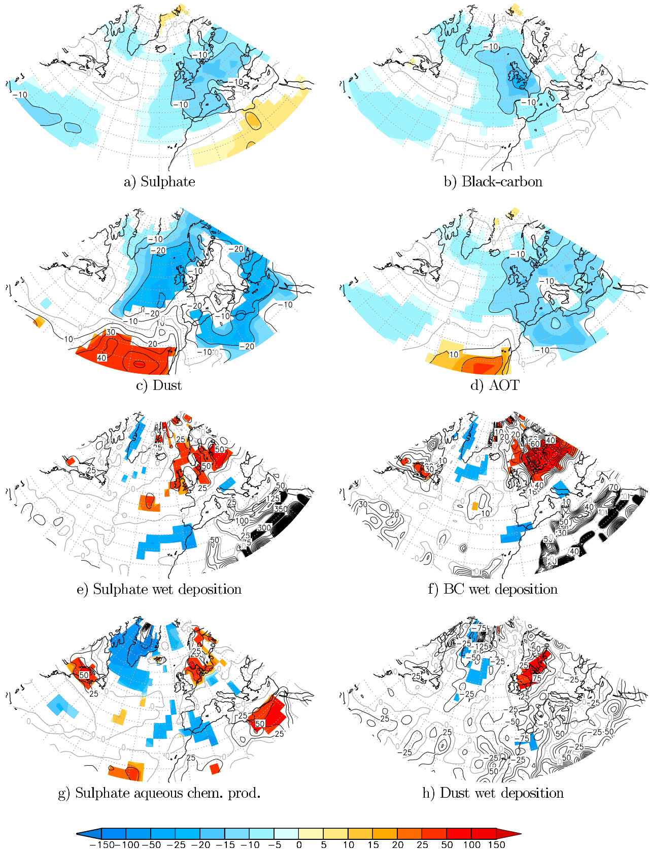
Figure 6. The 2000–2005 DJF zonal regime anomalies (in percentage) of sulfate burden, black carbon (BC) burden, dust burden, aerosol optical thickness (AOT), sulfate wet deposition, BC wet deposition, sulfate aqueous chemical production, and dust wet deposition over the North Atlantic region; 95% significant values are shown in color.
