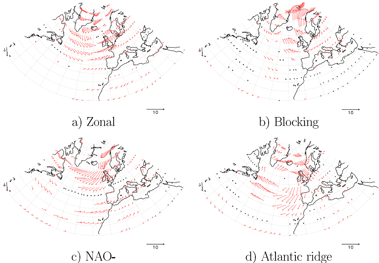
Figure 5. Composites of 2000–2005 ECMWF IFS model (see text for description) wind anomalies ( \text{m s}^{-1} ) during the days for which the atmosphere is classified as (a) zonal, (b) blocking, (c) NAO-, or (d) Atlantic ridge. The 95% significant values are shown in red.
