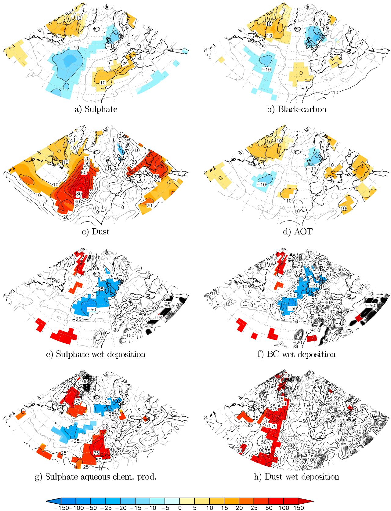
Figure 9. The 2000–2005 DJF Atlantic ridge regime anomalies (in percentage) of sulfate burden, black carbon (BC) burden, dust burden, aerosol optical thickness (AOT), sulfate wet deposition, BC wet deposition, sulfate aqueous chemical production, and dust wet deposition over the North Atlantic region; 95% significant values are shown in color.
