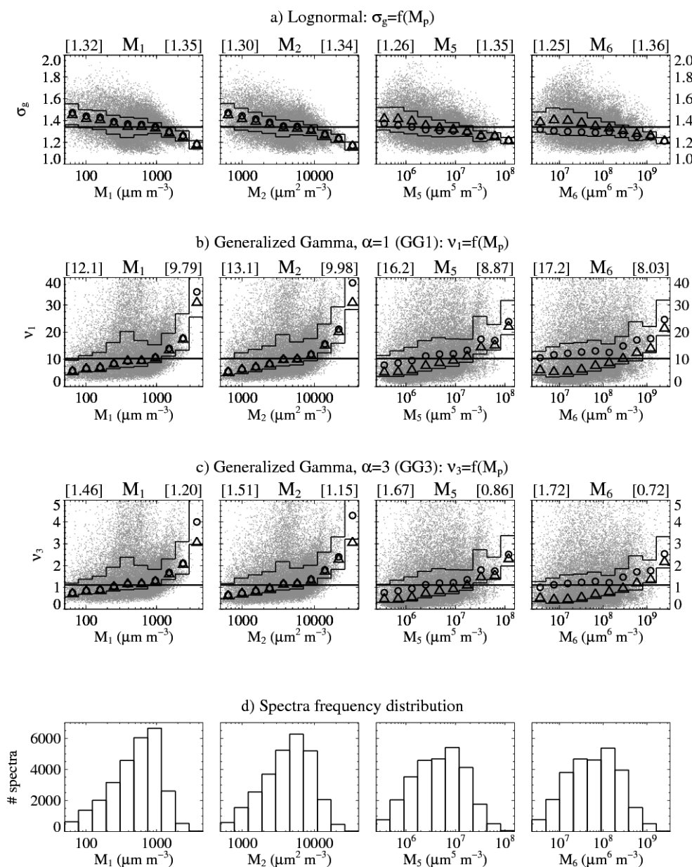
Fig. 2. Scatter-plots (grey points) of the tuning parameter values as a function, from left to right, of the M_1 , M_2 , M_5 , and M_6 moment values. The x-axis is divided in 10 classes on a Logscale. The thin lines denote the 25th and the 75th percentiles of the tuning parameter distribution in each class. The circles and triangles denote the tuning parameter value that minimizes the standard deviation of the absolute error and the geometric standard deviation of the relative error in each class, respectively. The horizontal thick line denotes the constant trade-off value of the tuning parameter. The top row is for the Lognormal function, the second and third rows are for the Generalized Gamma functions with \alpha=1 and \alpha=3 , respectively. On top of each graph, the number in brackets on the left (right) hand side is the tuning parameter value that minimizes the absolute (relative) error over the whole range of variation of the specified moment. The fourth row shows the number of sampled spectra in each moment class.
