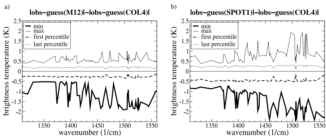
Figure 10. Minimum, maximum, first, and last percentiles of the brightness temperature differences between \text{lobs} - \text{guess} obtained with a new observation operator, (a) M12 or (b) SPOT1, and \text{lobs} - \text{guess} obtained with COL4 for clear IASI observations over western Mediterranean of September 2007 in all the WV channels studied displayed according to increasing wave number along the abscissa.
