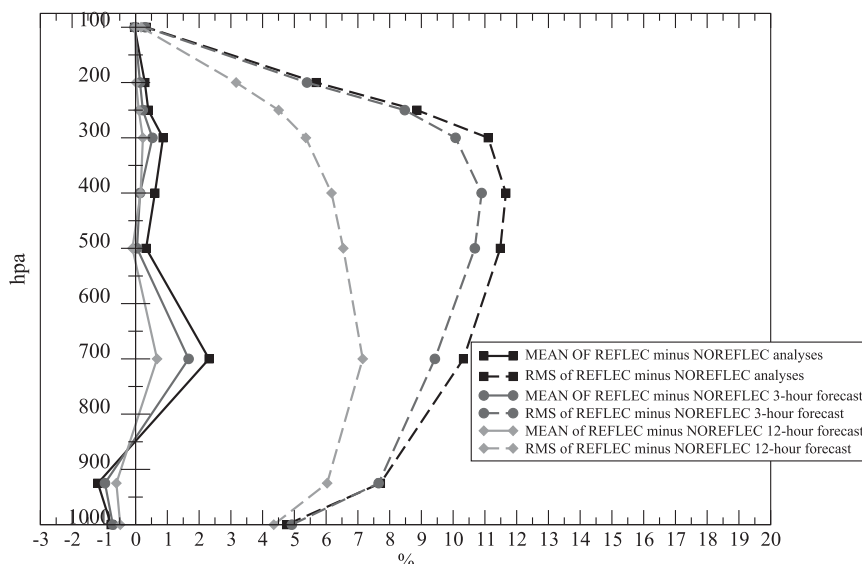
FIG. 6. Vertical profiles of analysis and forecast differences (mean and RMS) of relative humidity between REFLEC and NOREFLEC experiments for a 1-month average (11 Dec 2008–11 Jan 2009) over the AROME domain.
