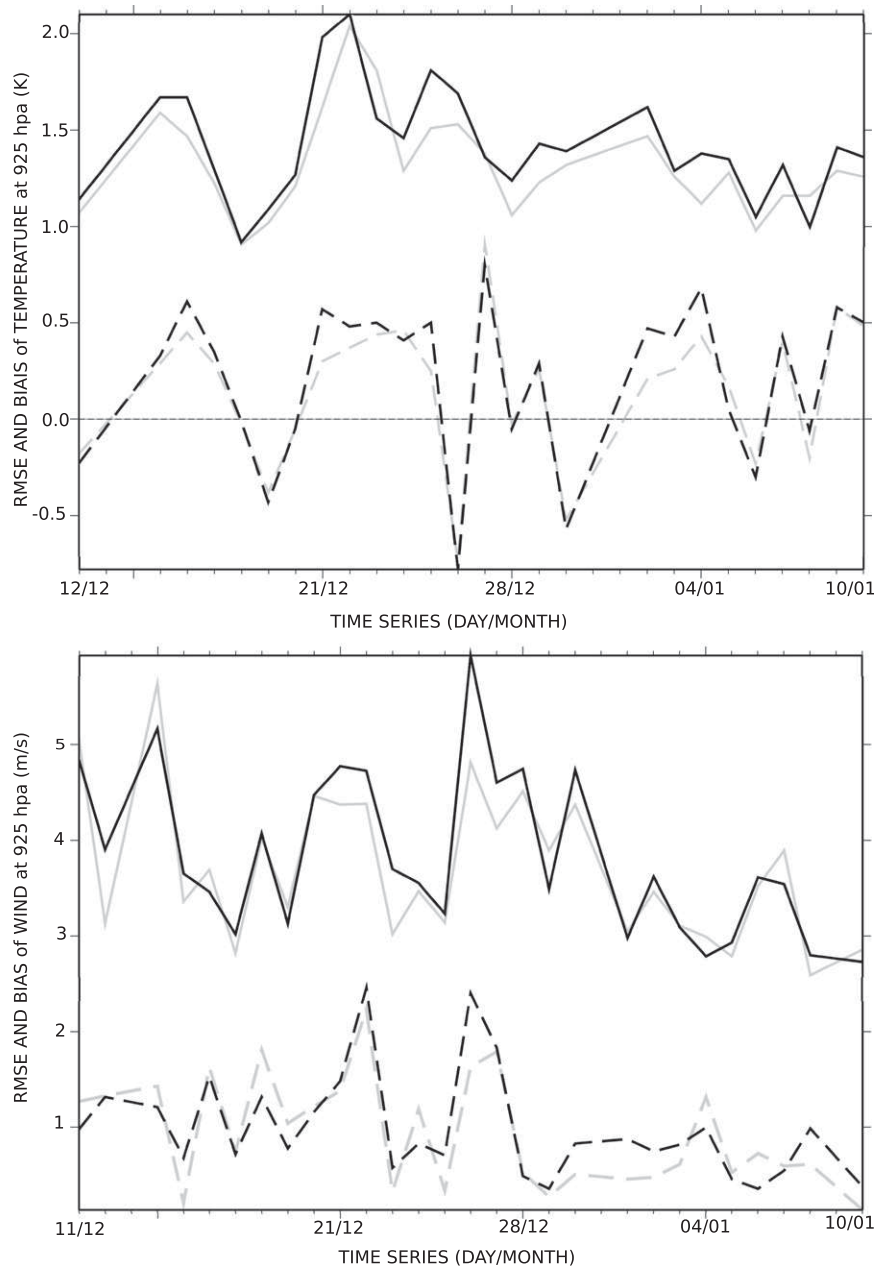
FIG. 10. Time series of RMS (solid lines) and bias (dashed lines) of the (top) 24-h forecast error in temperature at 925 hPa (forecasts errors are calculated with respect to own analysis) and (bottom) 12-h forecast error in wind at 925 hPa (forecasts errors are calculated with respect to radiosounding data), for REFLEC (gray lines) and NOREFLEC (dark lines), experiments between 12 Dec 2008 and 10 Jan 2009.
