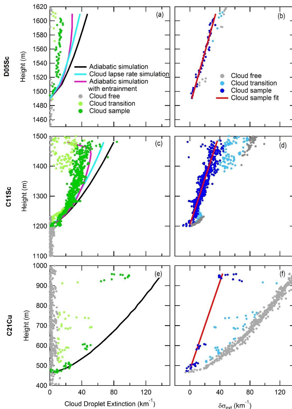
700 Figure 8. Vertical profiles of measured and simulated cloud extinction from flights D05Sc, C11Sc and C21Cu (left figures; Table 2). In-situ measurements are classified into cloud, cloud-transition and cloud-free observations. The difference between UAV-observed (green measurements) and ACPM-simulated cloud extinction (black line) on left figures are used 705 to calculate ( \Delta\sigma_{\text{ext}} ) as a function of altitude in the right-hand side figures. The slope of the best fit through in-cloud measurements (red line) represents the increase in \Delta\sigma_{\text{ext}} as a function of cloud thickness.
