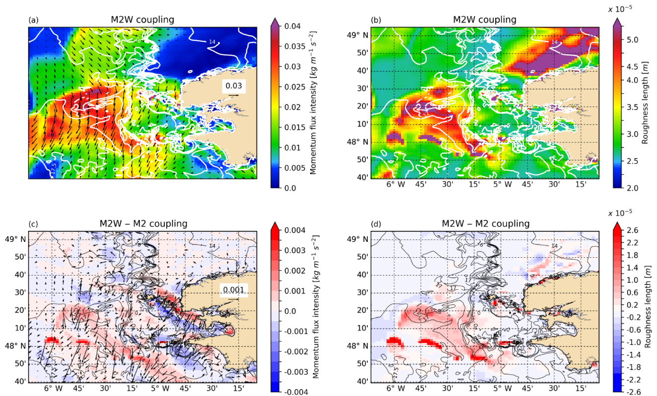
Figure 8. (a) Wind stress module (colour) and vector (arrows) (atmospheric sign convention), and SST (white contours with 0.5^{\circ}\text{C} interval) simulated by M2W. (b) Roughness length (colour) and SST (white contours with 0.5^{\circ}\text{C} interval) simulated by M2W. (c) Differences of the wind stress module (colour) and vector (arrows) when simulated by M2W versus M2. (d) Differences of the roughness length (colour) and the SST (black contours with 0.5^{\circ}\text{C} interval) simulated by M2W versus M2. All fields are shown at 09:00 UTC, 2 h after high tide.
