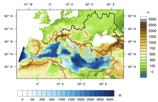
(b) CNRM-RCSM6
