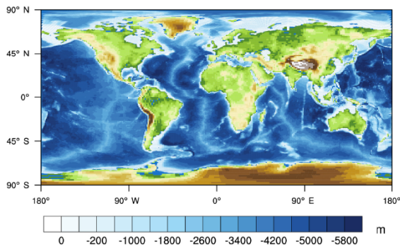
(a) CNRM-CM6
