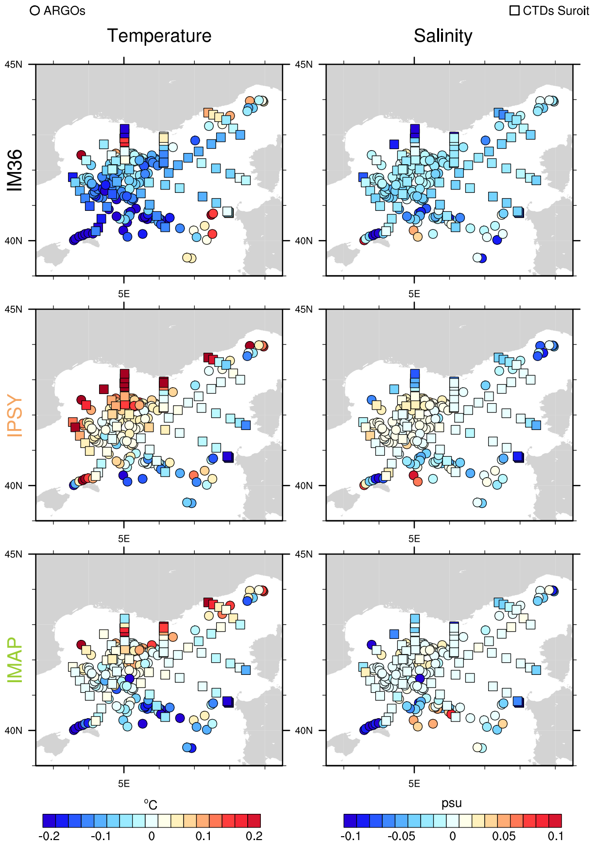
Figure 6. Vertically-averaged biases for temperature (left panels, °C) and salinity (right panels, psu) against in-situ profiles (ARGOs and R/V Le Suroit CTDs) for IM36 (top panels), IPSY (middle panels) and IMAP (bottom panels).
