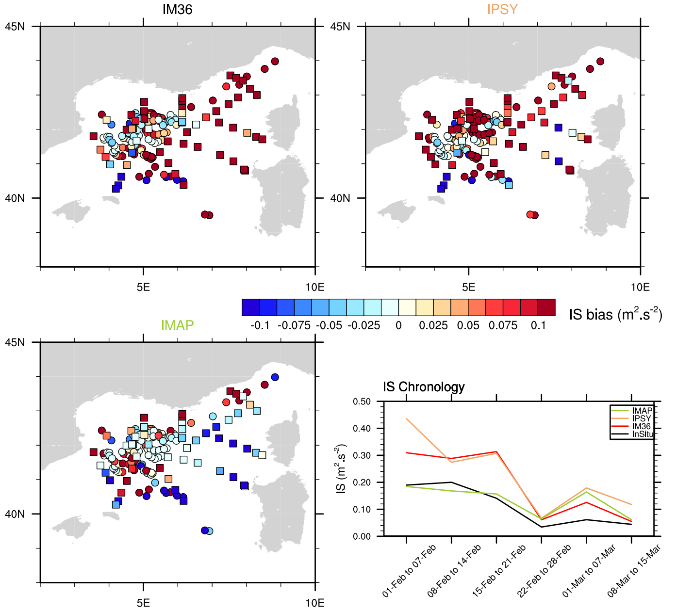
Figure 8. Index of Stratification (IS) biases ( m^2.s^{-2} ) against in-situ profiles (ARGOs and R/V Le Suroît CTDs) for IM36 (top left panel), IPSY (top right panel) and IMAP (bottom left panel). Bottom right panel: observed and simulated IS time-series during SOP2.
