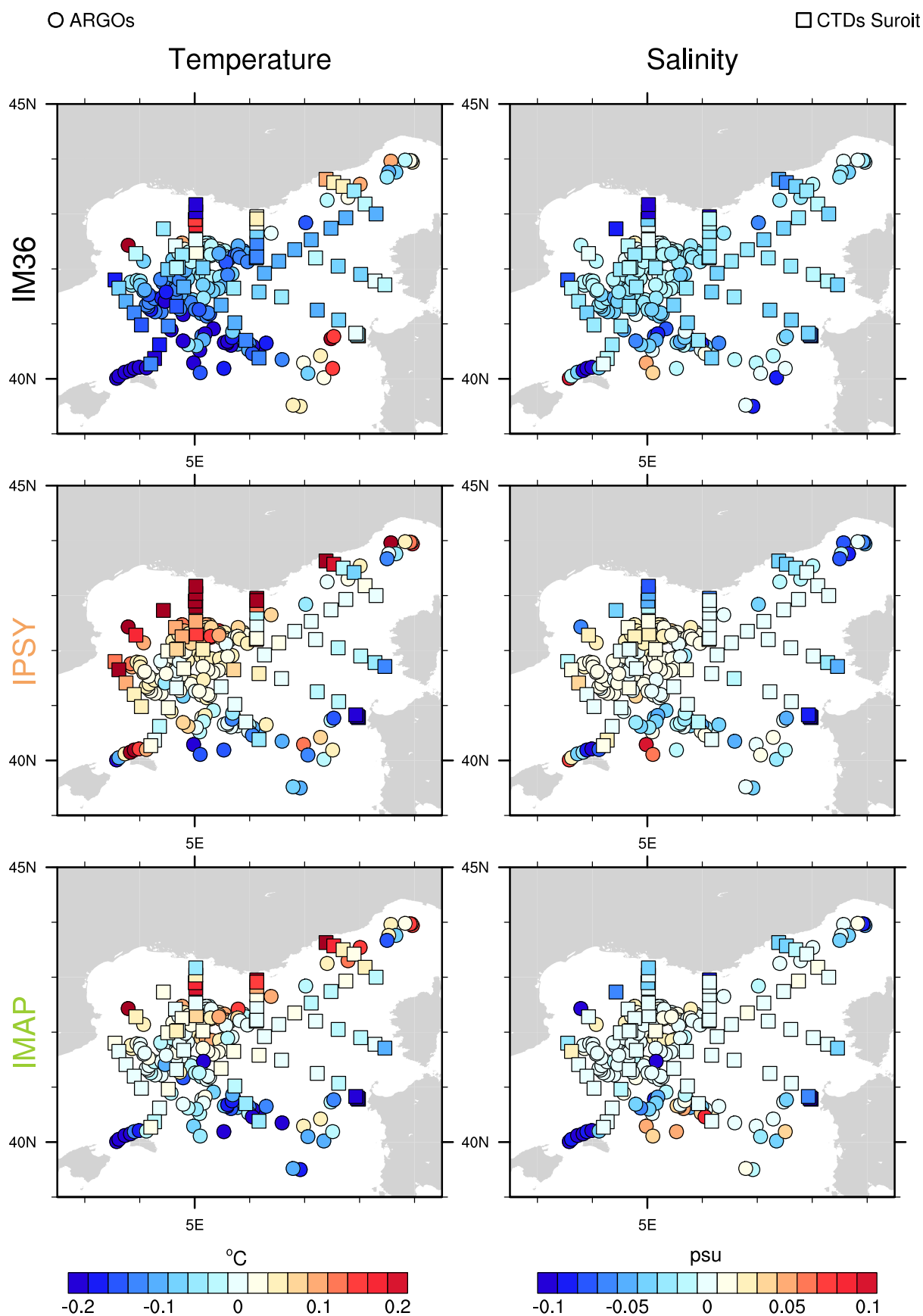
Figure 6. Vertically-averaged biases for temperature (left panels, °C) and salinity (right panels, psu) against in-situ profiles (ARGOs and R/V Le Suroît CTDs) for IM36 (top panels), IPSY (middle panels) and IMAP (bottom panels).
