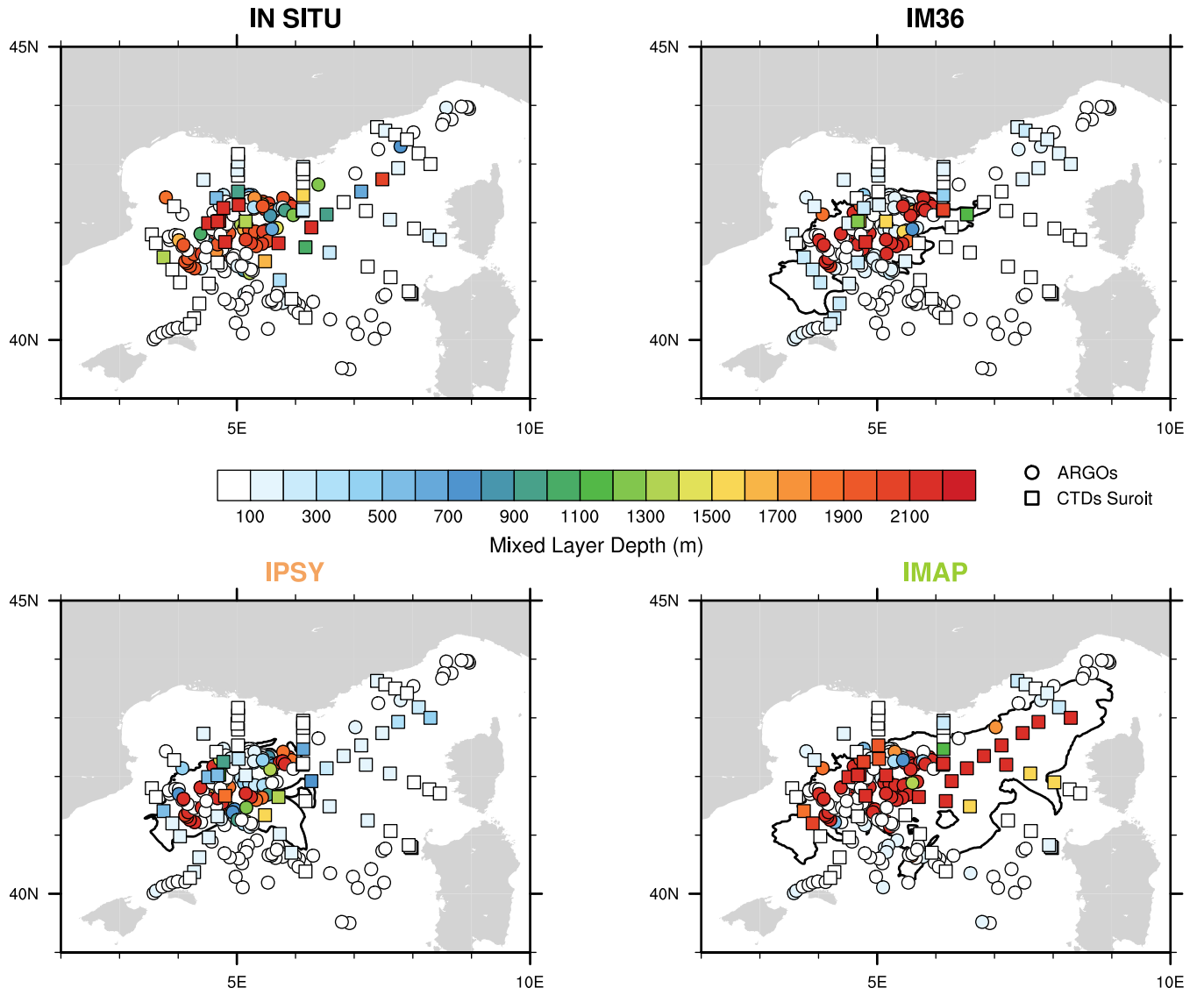
Figure 9. Mixed layer depth (meters) from density in-situ profiles (ARGOs and R/V Le Suroît CTDs) and colocalized simulated MLD (density criteria) in IM36, IPSY and IMAP. Contours indicate area where the maximum MLD goes deeper than 2000 meters during SOP2 in the simulations.
