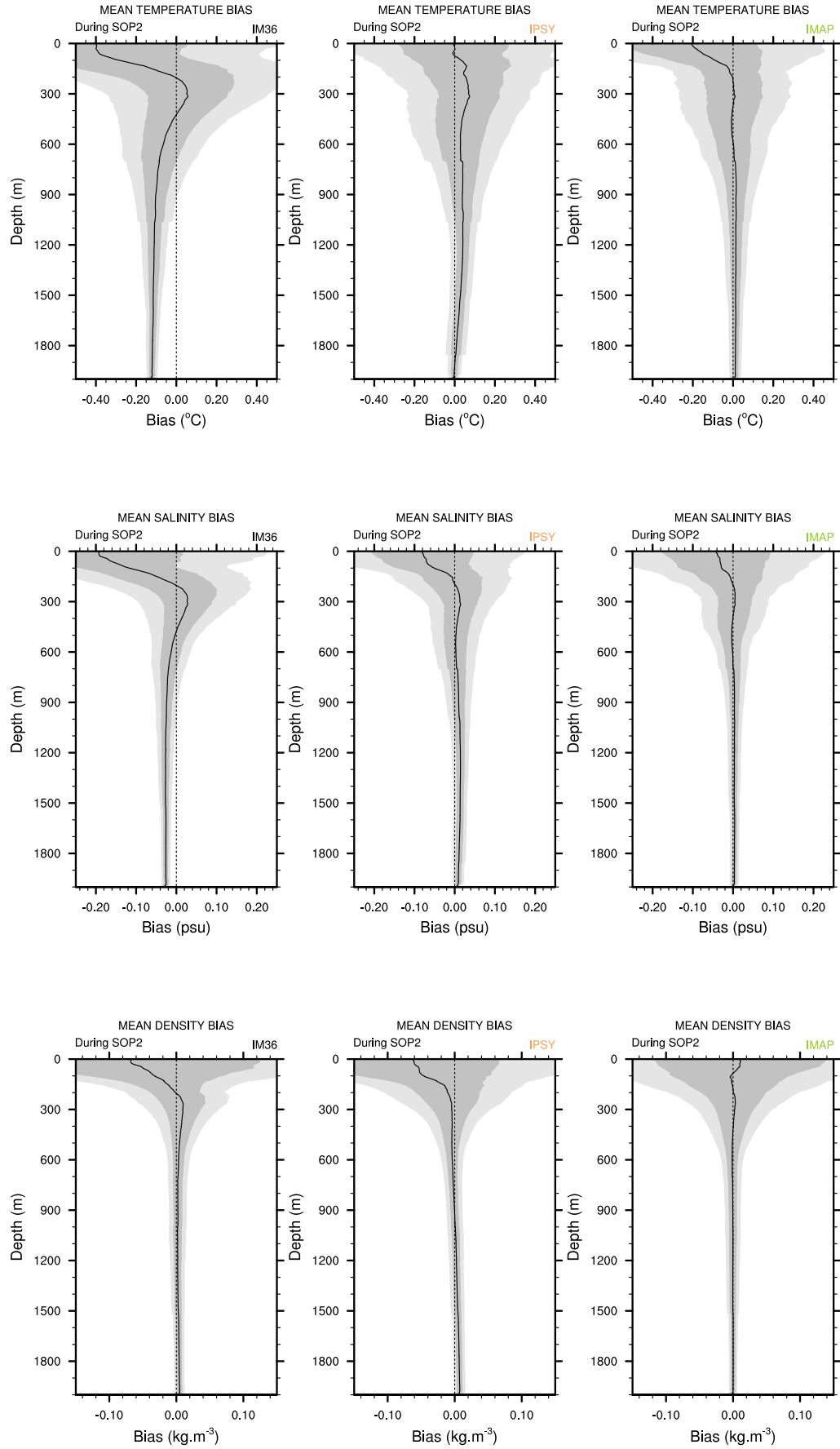
Figure 5. Mean vertical biases in temperature (°C), salinity (psu) and density (kg.m -3 ) against the ARGO dataset of the whole SOP2, for the three experiment IM36, IPSY and IMAP. The darkgrey area is \pm\sigma ; the lightgrey area is for \pm2\sigma .
