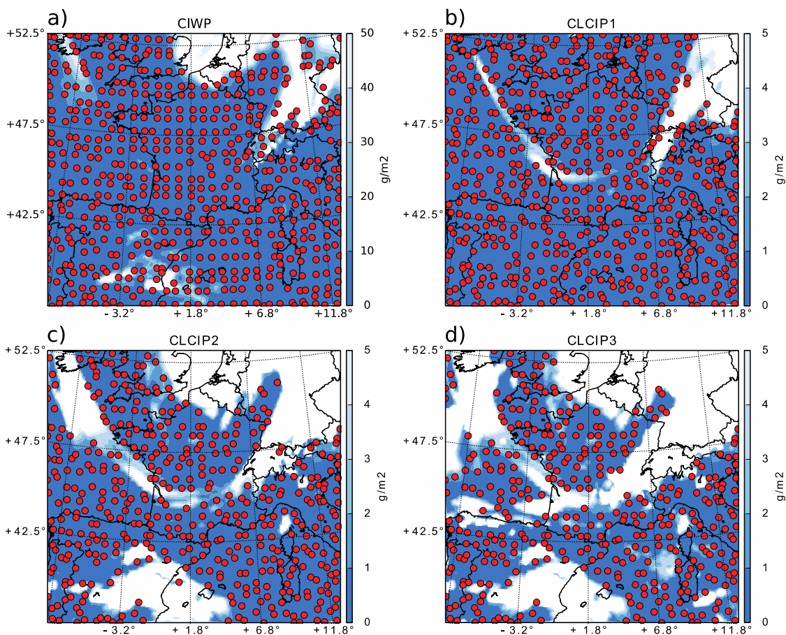
Figure 5: Example of MWGEO and IRS active observations after cloud screening (circles) for July 3 rd , 2015 at 00 h UTC. (a): channel 4 of the MWGEO peaking at 550 hPa and threshold on CIWP of 30 \text{ g m}^{-2} , (b) channel 978 of the IRS peaking at 150 hPa and threshold on CLCIP1 of 2 \text{ g m}^{-2} , (c) channel 1130 of the IRS peaking at 350 hPa and threshold on CLCIP2 of 2 \text{ g m}^{-2} , (d) channel 1260 of the IRS peaking at 600 hPa and threshold on CLCIP3 of 2 \text{ g m}^{-2} . The Nature Run cloud screening parameter for each channel is plotted in background.
