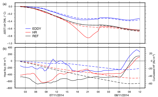
Figure 11. Time series of the SST (solid line) and potential temperature in the OML (dashed line) (a) and instantaneous (solid line, left-hand-side scale) and integrated downward heat flux (dashed line, right-hand-side scale) (b) in the EDDY (blue), HR (red), and REF (black) zones (see text).
