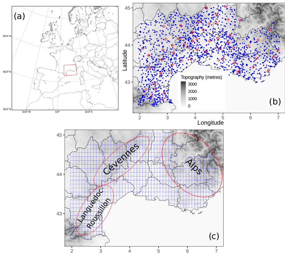
Figure 1. Panel (a) shows a situation map of the investigated area (rectangle with red edges) with respect to western Europe and the Mediterranean Sea. Panel (b) shows the rain-gauge network used for the study. Red diamonds represent the rain gauges selected for cross-validation testing, and blue dots represent the rain gauges selected for cross-validation training. Panel (c) shows the 0.1^{\circ} \times 0.1^{\circ} model grid (in blue), along with the location of three key areas. Domain D is located within the borders of the model grid (c).
