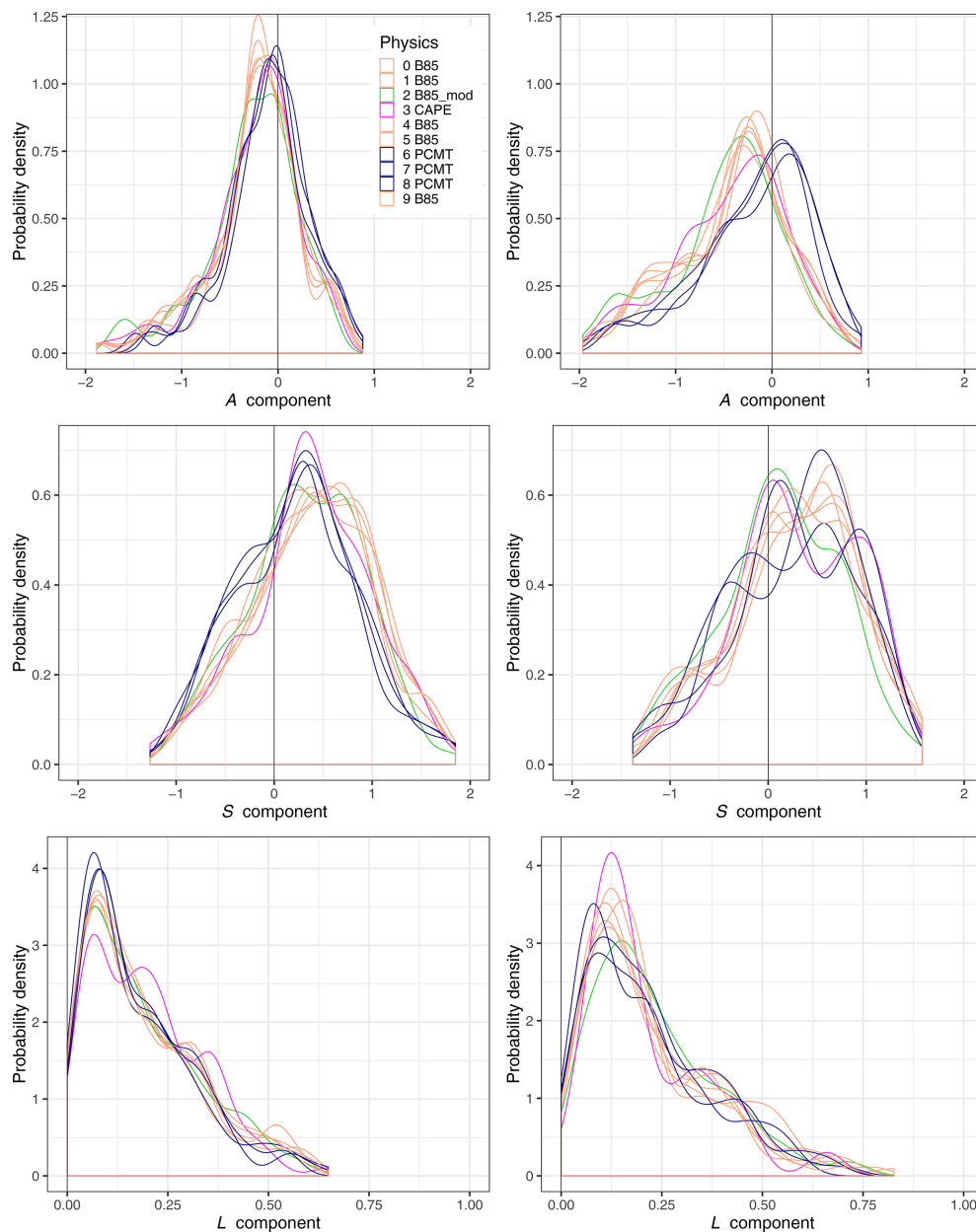
Figure 8. Probability density functions of the three SAL components for the HPEs and for each physics of the reforecast system (coloured lines). Physics scheme are gathered in four categories depending on the parametrization of the deep convection: PCMT (blue), B85 (orange), B85 mod (green), and CAPE (purple). The left column corresponds to lead time LT12, and the right column relates to lead time LT34.
