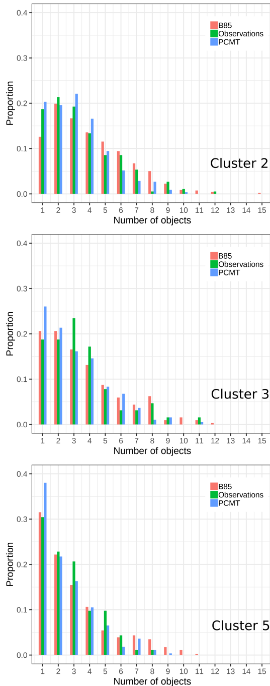
Figure 11. Normalized histograms of the daily number of SAL patterns, for the B85 physics scheme (red), PCMT (blue), and observation (green). Panels correspond to the three-cluster classification.
