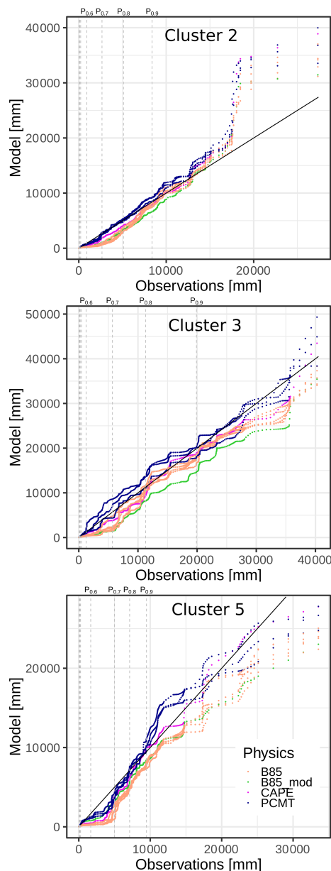
Figure 13. Quantile–quantile plot between SAL pattern rain amounts from the model (Y axis) and from the observation (X axis). Physics schemes are gathered into four classes (B85, PCMT, B85 mod , CAPE). Observation deciles correspond to the vertical dashed lines.
