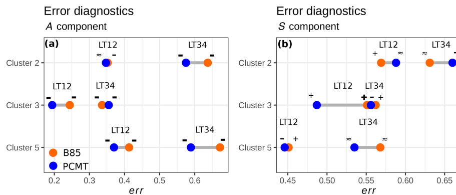
Figure 10. Dumbbell plot of integrated error diagnostics computed using Eq. (11). Colours refer to B85 (orange) and PCMT (blue) deep-convection parametrization schemes. Results are stratified on the basis of the clusters and lead times. Symbols denote whether positive or negative errors dominate. These signs are defined using the following definition: - (bold) if \frac{\text{err}_-}{\text{err}_+} \geq 2 ; - (bold) if 1.1 \leq \frac{\text{err}_-}{\text{err}_+} < 2 ; \approx if 0.9 < \frac{\text{err}_-}{\text{err}_+} < 1.1 ; + (bold) if 0.5 < \frac{\text{err}_+}{\text{err}_-} \leq 0.9 ; + (bold) if \frac{\text{err}_+}{\text{err}_-} \leq 0.5 .
