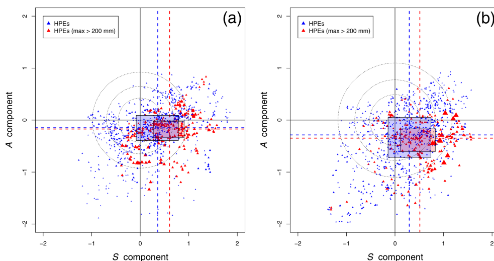
Figure 6. Relationship between the A component and the S component of the SAL score (SAL diagrams) for HPEs only, for lead times LT12 (a) and LT34 (b). Blue triangles represent HPEs with grid-point maximum rainfall under 200 \text{ mm d}^{-1} , and red triangles show rainfall amounts above 200 \text{ mm} . Triangles are proportional to the rainfall value. Some main characteristics of the component distribution are plotted. The median value is shown as dashed lines, and percentiles 25 and 75 delimitate the boxes. Circles represent the limits 25th, 50th, and 75th percentiles to the best score ( A = 0 , S = 0 ).
