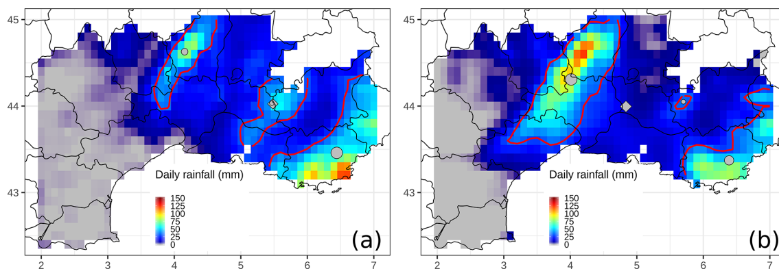
Figure 4. SAL pattern analysis for the case of 28 October 2004, applied to the observation data (a) and one 60 h lead time forecast (b). Base contours of the identified objects are shown as red lines. Grey points stand for the rain barycentre of each pattern, and the grey diamond depicts the rain barycentre for the whole field. The size of the barycentre points is proportional to the integrated mass of the associated object.
