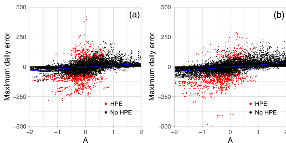
Figure 5. Relationship between the daily rainfall grid-point maximum algebraic error and the A component of the SAL score. HPE days are plotted in red, while other days are in black. Panel (a) is for LT12 lead time, and (b) shows LT34 lead time. Linear regression analysis is added to the plot.
