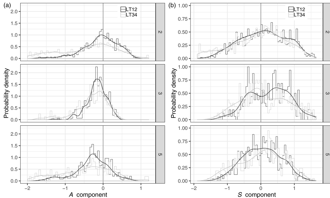
Figure 7. A-component (a) and S-component (b) normalized histograms and probability density functions for clusters 2, 3, and 5. Results for lead time LT12 are plotted as black lines, and results for lead times LT34 are in grey.
