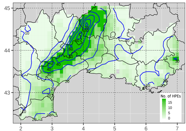
Figure 2. Annual average of HPE occurrence per grid point (in green). The composite of daily rainfall amounts ( \text{mm d}^{-1} ) of the HPE dataset is represented by the blue isohyets.
