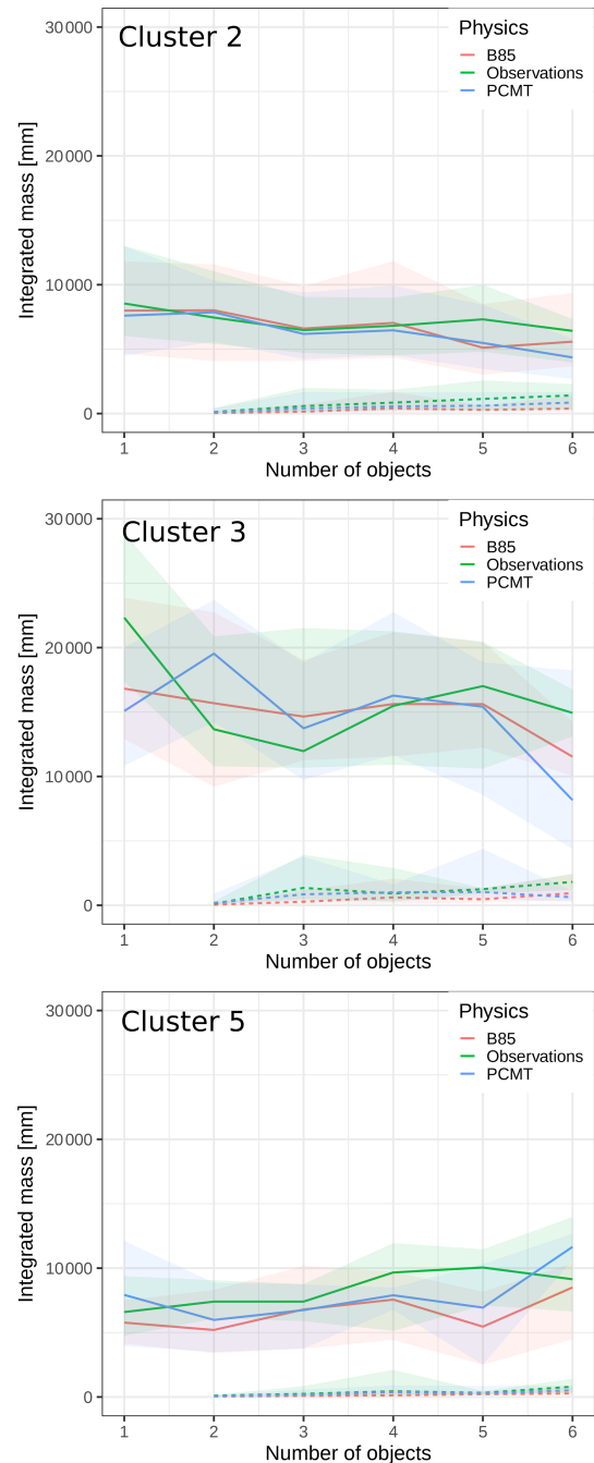
Figure 12. Distribution of the SAL first-pattern O_1 rain amount according to the number of patterns per day. Curves stand for the median of the distribution, and shaded areas range between the 25th and 75th percentiles. The dashed lines correspond to the second ranked SAL pattern O_2 rain amount.
