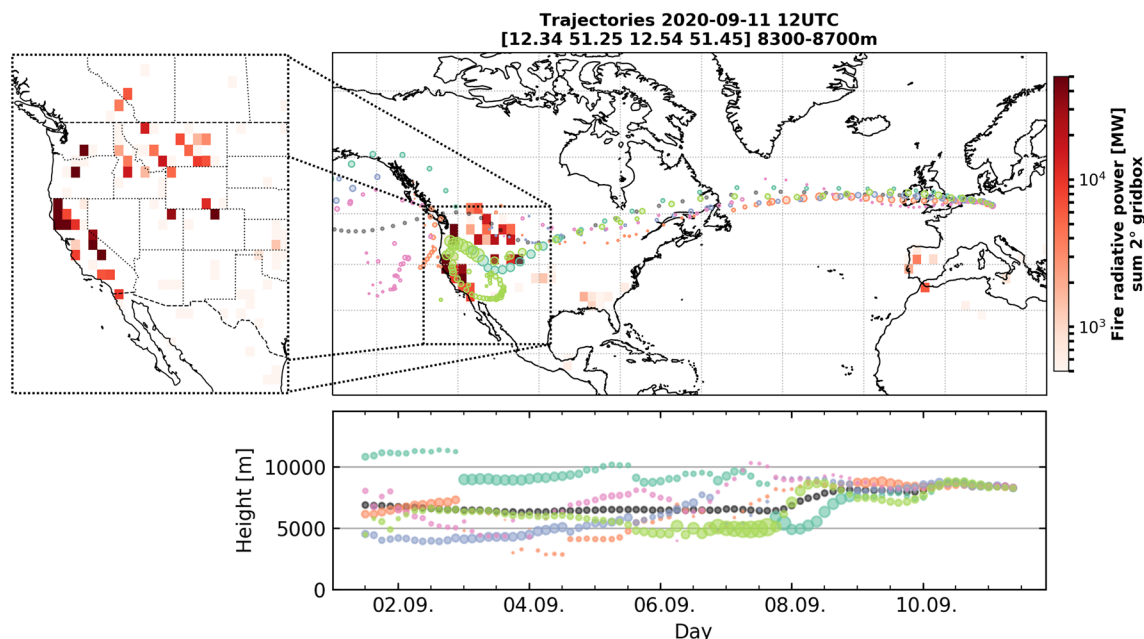
Figure 2. Air-mass origin at Leipzig on September 11, 2020 underlaid with MODIS derived fire radiative power: Clusters of air parcel positions ending at Leipzig between 8.3 and 8.7 km height at 12 UTC (see text for further description). Geographic location (top panel) and heights (bottom panel) of the clusters (indicated by color) are shown. Dot size denotes the size of each cluster. Dark gray dots denote the mean position of all particles. MODIS derived fire radiative power was gridded to 2°. Only fire detections between 31 August and September 7, 2020 are included. A zoomed map of the fire radiative power gridded to 1° in the western US is shown at the left.
