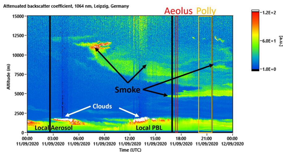
Figure 1. Time-height plot of the uncalibrated attenuated backscatter coefficient at 1064 nm measured at ground in Leipzig, Germany, with the multiwavelength-Raman polarization lidar PollyXT. The time of the overpass is indicated as red rectangle while the data analysis period of the ground-based lidar data is highlighted in orange. No data is available during regular depolarization calibrations (black).
