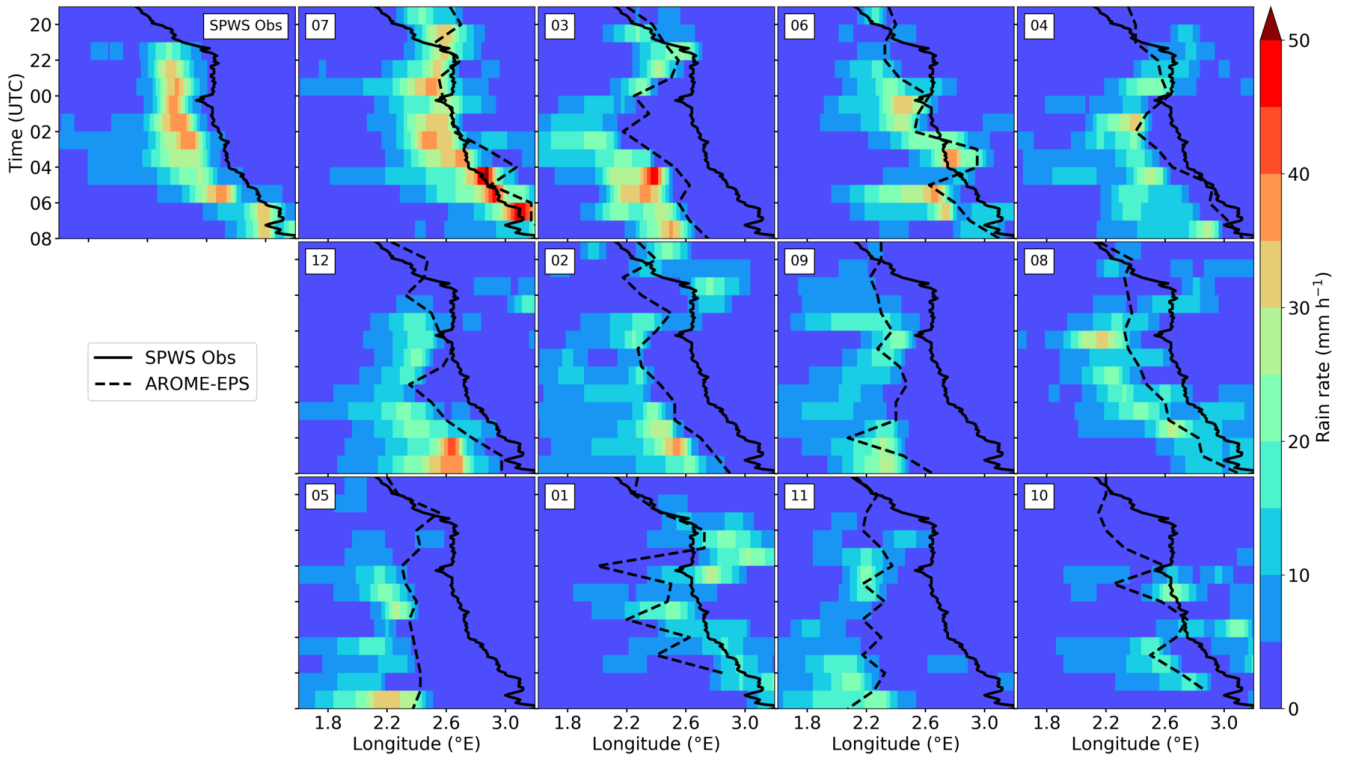
Figure 16. Hovmöller diagram of the mean trough’s longitude over the Aude valley observed with SPWS analyses and predicted by the members of the AROME-EPS between 19:00 UTC on 14 October and 08:00 UTC on 15 October. The mean hourly rain rate observed by SPWS ANTILOPE or predicted by AROME-EPS over the Aude valley [43.15–43.33° N] is shown as a function of the longitude. Members are ranked as in Fig. 9.
