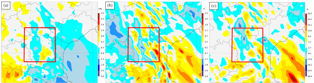
Figure 10. Average difference of the three most rainy AROME-EPS members based on 15:00 UTC analysis on 14 October. The forecast time is 02:00 UTC on 15 October 2018, i.e. in the middle of the period of interest. The anomaly is computed with respect to the ensemble mean at each point. (a) Mean sea level pressure (hPa), (b) moist potential temperature \theta'_w (K) at 850 hPa, and (c) relative humidity (%) at 850 hPa.
