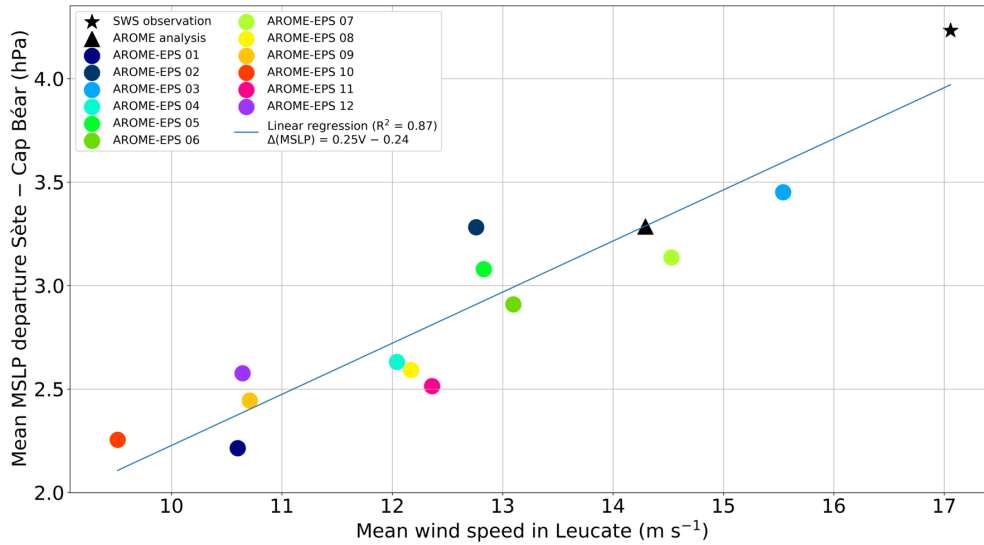
Figure 13. SWS observation, AROME–France analysis, and AROME–EPS forecasts of 10 m wind speed blowing from the Mediterranean Sea (sector 90–150°) as a function of the MSLP departure between Sète and Cap Béar, averaged over the event between 19:00 UTC on 14 October and 07:00 UTC on 15 October (period taken 1 h ahead of the period of interest). To give an order of magnitude, if we hypothetically consider that the geostrophic balance applies near the ground, the ageostrophic wind is equal to zero, and the pressure field is such that the Sète–Cap Béar orientation is always parallel to the pressure gradient during the event, the slope of the regression line would theoretically be about 0.13 (with a y intercept equal to zero).
