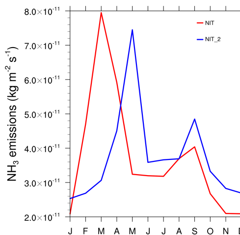
Figure 2. 1979–2016 monthly means of \text{NH}_3 emissions ( \text{kg m}^{-2} \text{ s}^{-1} ) over Europe as defined in Fig. 1, used for NIT (red, based on MACCity) and NIT_2 (blue, from CMIP6) simulations. The annual total is equal in the two versions ( 4.5 \times 10^{-10} \text{ kg m}^{-2} \text{ s}^{-1} ).
