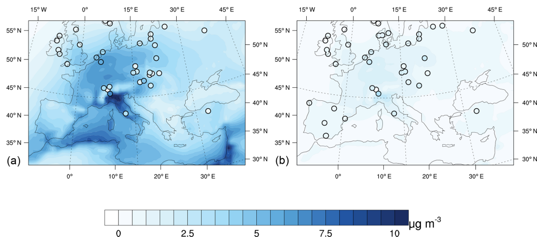
Figure 4. Nitrate (a) and ammonium (b) surface concentration ( \mu\text{g m}^{-3} ) simulated by the ALADIN-Climat model (1994–2014) and measured at EMEP stations (coloured dots) using the same colour palette.
