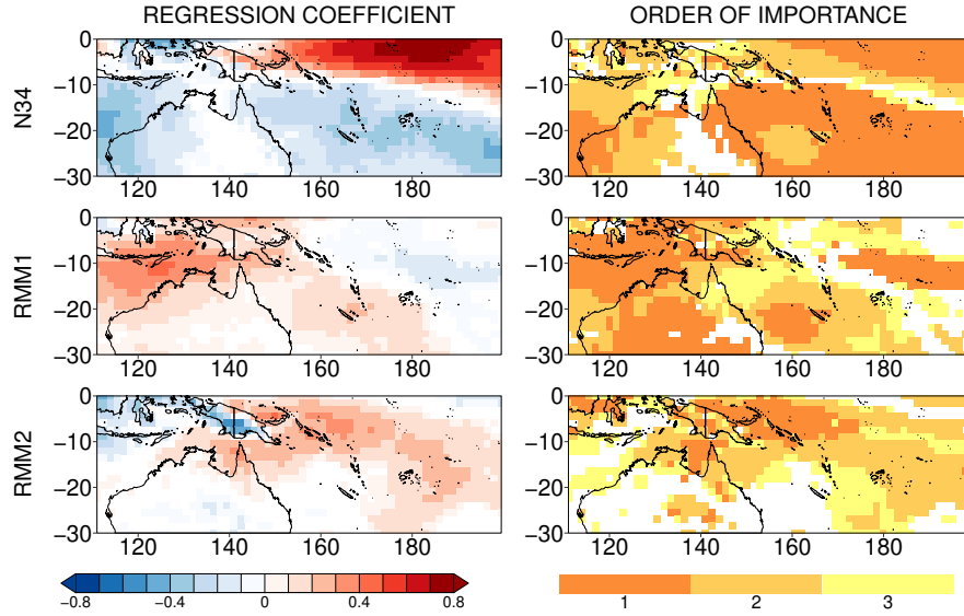
Fig. 7 Left: linear regression coefficient of each predictor against observed rainfall \hat{r}_o . Grid points are in white if the coefficient is not significant at the 95% level. Right: Order of selection for each predictor in a stepwise forward selection scheme when considering large-scale predictors only in reference data. Grid points in white correspond to grid points where adding the predictor leads to a p-value greater than 0.05 in the likelihood-ratio test.
