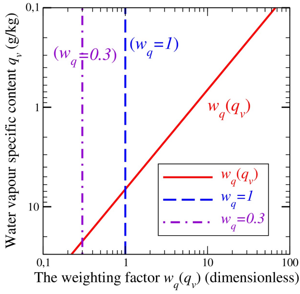
Figure 7: The dimensionless exergy weighting factor w_q(q_v) given by (19) plotted with q_v in ordinates.
