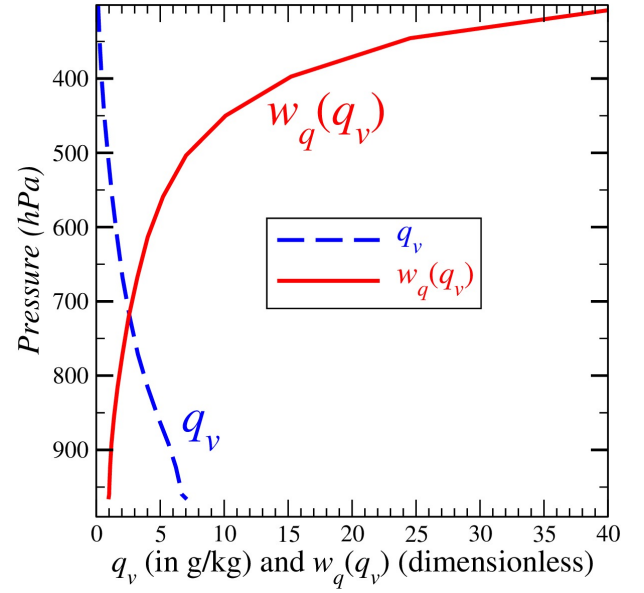
Figure 8: The dimensionless exergy weighting factor w_q(z) given by (19) for the vertical profile of average values \overline{q_v}(p) of the GEM-CMC dataset used to plot the Fig. 6c.
