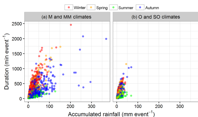
Figure 4. Rainfall duration vs. accumulated rainfall across seasons for each marked rainfall event at Mediterranean (M) and Mediterranean–mountain (MM) stations (a) and at oceanic (O) and semi-oceanic (SO) stations (b).
