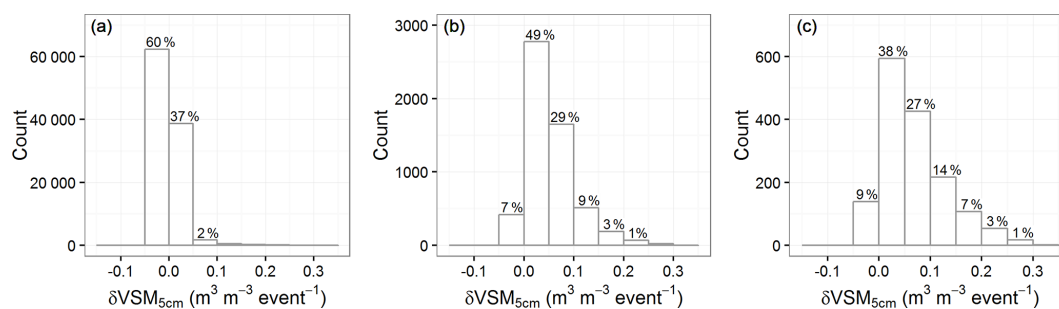
Figure 9. Statistical distribution of \delta VSM_{5\text{cm}} for 104 178 fully documented rainfall events (a), 5714 marked rainfall events (b), and 1577 marked rainfall events affecting topsoil temperature (c) defined in Table 2.
