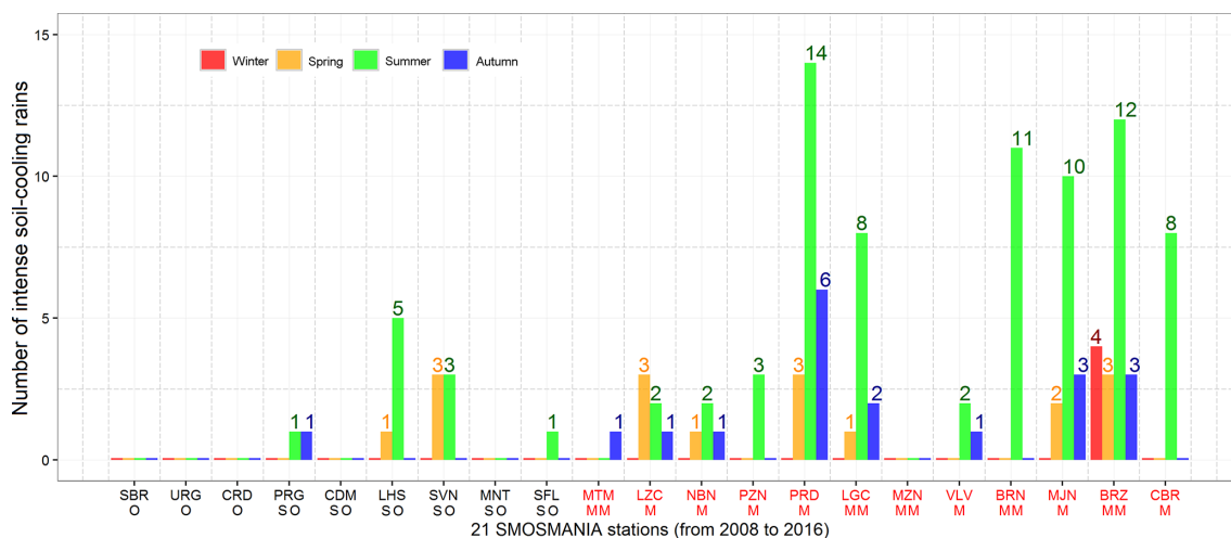
Figure 6. Statistical distribution of the 122 intense soil-cooling rains among stations of the SMOSMANIA network across seasons. Red, orange, green, and blue bars are for winter, spring, summer, and the autumn, respectively. Symbols “O”, “SO”, “M”, and “MM” indicate oceanic, semi-oceanic, Mediterranean, and Mediterranean–mountain climates, respectively. Stations are listed from (left) west to (right) east.
