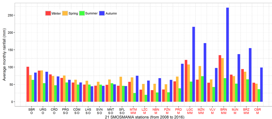
Figure 3. Average monthly rainfall (in units of mm) for the 21 SMOSMANIA stations across seasons from 2008 to 2016. Stations are sorted from (left) west to (right) east. Symbols “O”, “SO”, “M”, and “MM” indicate oceanic, semi-oceanic, Mediterranean, and Mediterranean–mountain climates, respectively. Winter season is from December to February.
