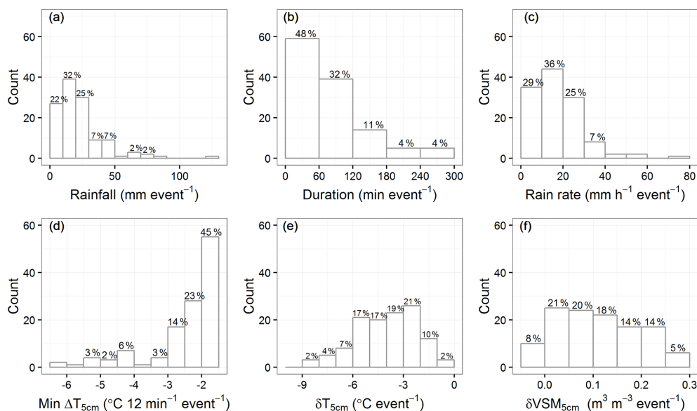
Figure 7. Statistical distribution of the 122 intense soil-cooling rains in terms of (Sect. 3.3) accumulated rainfall (a), rain duration (b), rain rate (c), minimum \Delta T_{5\text{cm}} (d), \delta T_{5\text{cm}} (e), and \delta \text{VSM}_{5\text{cm}} (f), with bins of 10 mm, 60 min, 10 mm h -1 , 1 °C, 1 °C, and 0.05 m 3 m -3 , respectively.
