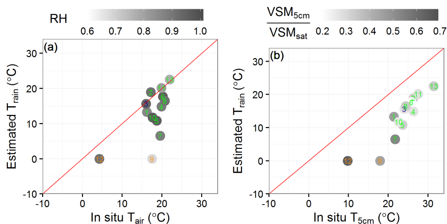
Figure 8. Estimated T_{\text{rain}} for the 13 cases listed in Table 5 vs. observed ambient T_{\text{air}} (a) and observed T_{5\text{cm}} (b), with levels of grey indicating air relative humidity (RH, dimensionless) and \text{VSM}_{5\text{cm}} to \text{VSM}_{\text{sat}} ratio (dimensionless) values at time t_1 .
