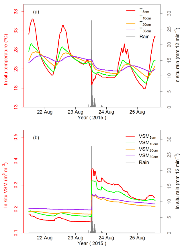
Figure 2. In situ soil temperature (a) and soil moisture (b) measured at the PRD station from 21 to 25 August 2015 at depths of 5, 10, 20, and 30 cm, together with the in situ rainfall observations ( \text{mm } 12\text{ min}^{-1} ) shown in grey.
