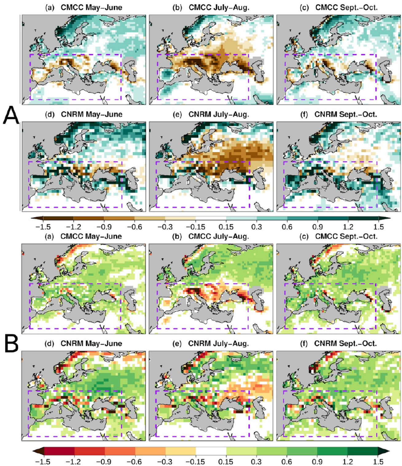
Fig. 4 A Two-month precipitation bias against GPCC (1961–2010), in mm/day and B difference between bi-monthly model precipitation standard deviation and absolute value of the precipitation bias against GPCC (1961–2010), in mm/day
