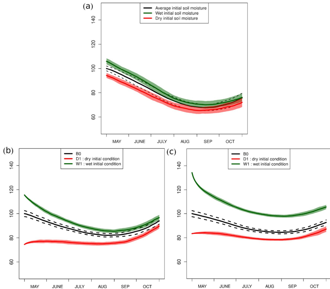
Fig. 6 Top first meter soil moisture evolution over MED with initial wet (green), dry (red) and average (black) conditions, based on ensembles from the ERA-20C composites analysis ( a ) and CNRM ( b ) and CMCC ( c ) simulations, in % of the average ensemble mean
