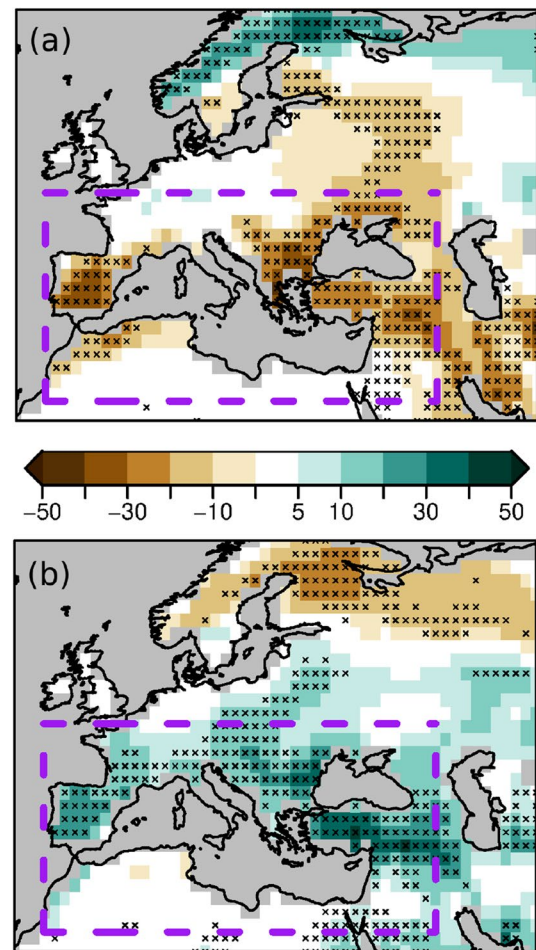
Fig. 2 Top first meter soil water content anomalies on May 1st, in \text{kg}/\text{m}^2 for dry (a) and wet (b) composites in the ERA-20C reanalysis. Stippling indicates significant anomalies at the 95% confidence level. The MED domain is outlined by the purple dashed box
