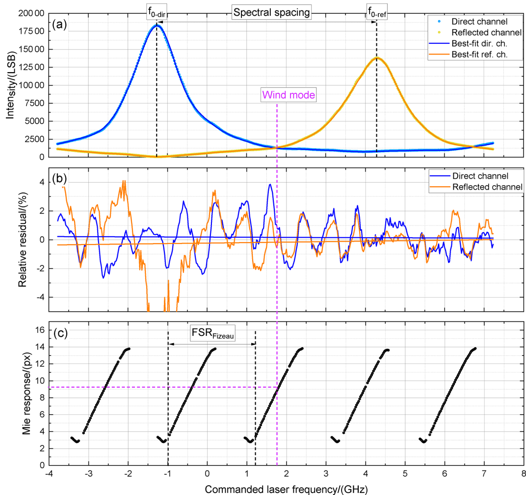
Figure 5. (a) FPI transmission curves of the direct channel (light-blue dots) and the reflected channel (yellow dots) measured on 10 October 2018, laser-energy-corrected by means of E_{\text{norm}_{\text{new}}}(f) (see also Eq. 2), and the corresponding best fits according to Eqs. (9) and (11) in blue (direct channel) and orange (reflected channel), respectively. (b) Related relative residuals of the direct channel (blue) and reflected channel (orange). (c) Corresponding Mie response, i.e., the fringe center position on the ACCD pixel.
