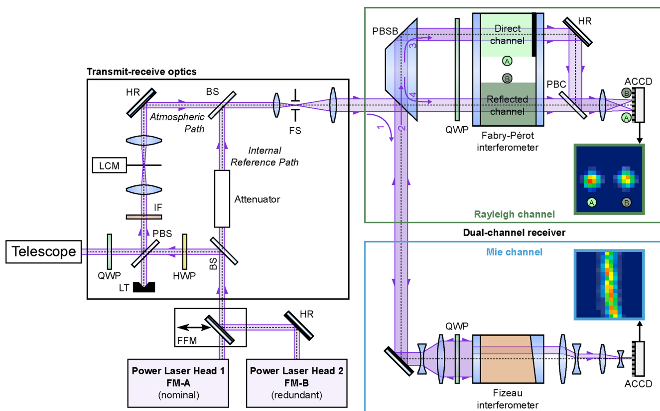
Figure 1. Sketch of the ALADIN optical receiver layout reproduced from Lux et al. (2021). QWP: quarter-wave plate; HWP: half-wave plate; PBS: polarizing beam splitter; PBSB: polarizing beam splitter block; PBC: polarizing beam combiner; FFM: flip-flop mechanism; BS: beam splitter; HR: high-reflectance mirror; LCM: laser chopper mechanism; FS: field stop; IF: interference filter; LT: light trap; ACCD: accumulation charge-coupled device.
