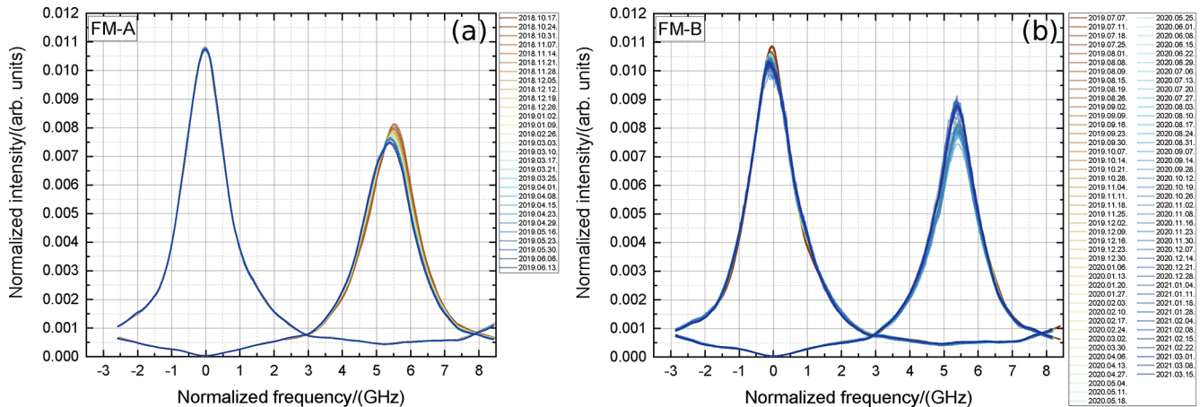
Figure 6. Normalized FPI transmission curves acquired during ISR measurements performed from 10 October 2018 to 15 March 2021 (see also Table 2) for the FM-A period (October 2018 to June 2019, a ) and FM-B period (July 2019 to March 2021, b ).
