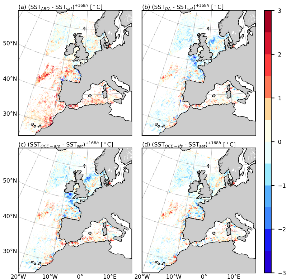
Figure 4. Comparison with L3 satellite SST observations at the end of the simulation (19 October 2018, 00:00 UTC) : differences ( ^{\circ}\text{C} ) with (a) ARO SST, (b) OA simulated SST, (c) OCE-aro simulated SST and (d) OCE-ifs simulated SST.
