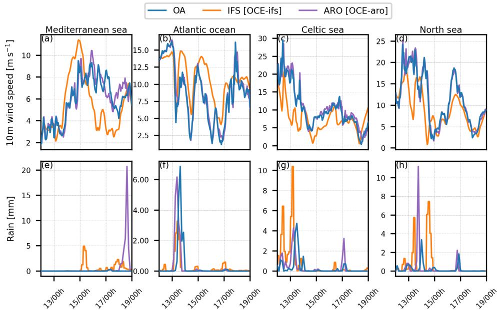
Figure 13. Temporal evolution of simulated 10 m wind speed ( m s^{-1} ; a, b, c, d) and rainfall ( mm h^{-1} ; e, f, g, h) extracted in the four areas presented in Fig. 3d.
