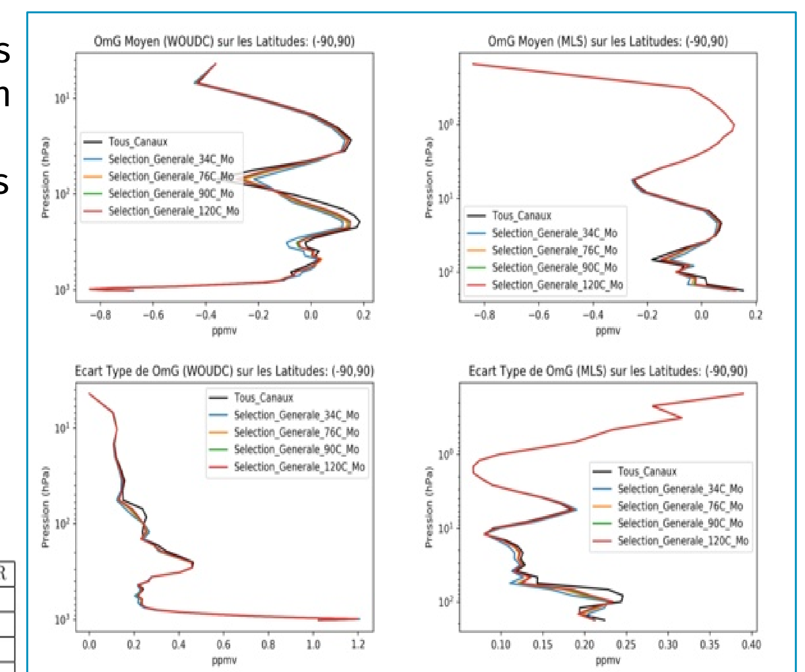
Fig 3: Vertical profiles of scores wrt WUOUC (left) and MLS (right), for biases (top) and standard deviations (bottom).
