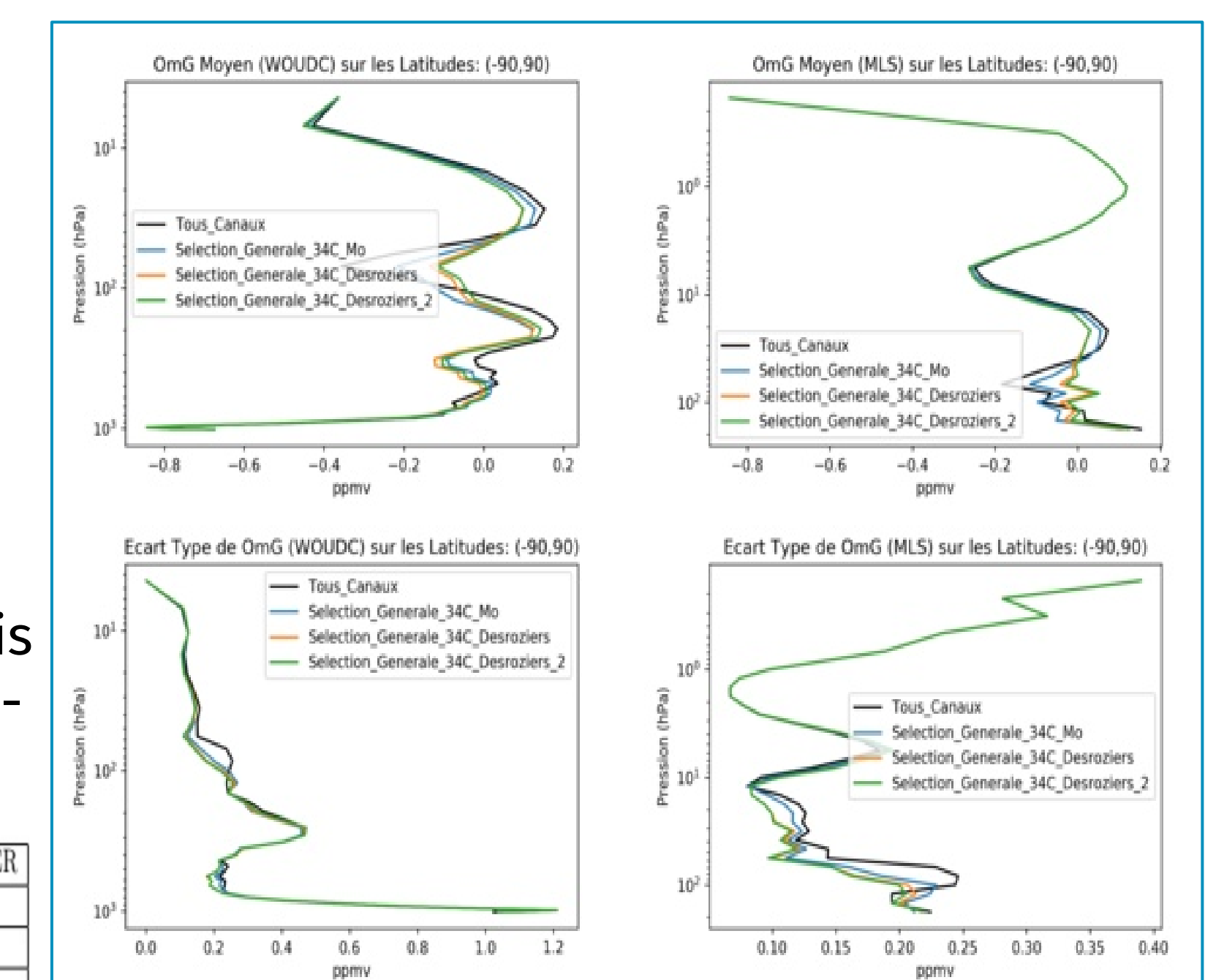
Fig 6: Vertical profiles of scores wrt WUOUC (left) and MLS (right), for biases (top) and standard deviations (bottom).
