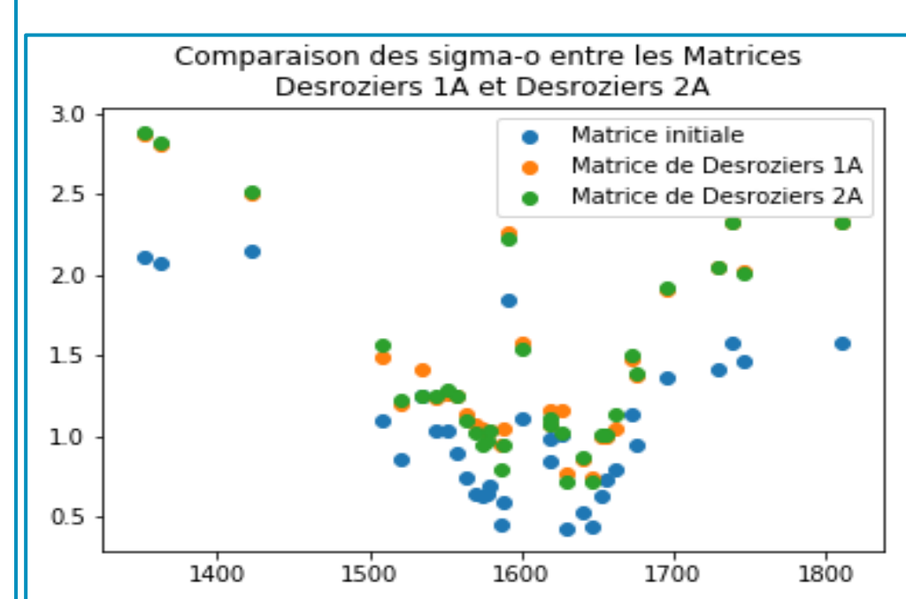
Fig 5: Initial and diagnosed sigma-o
