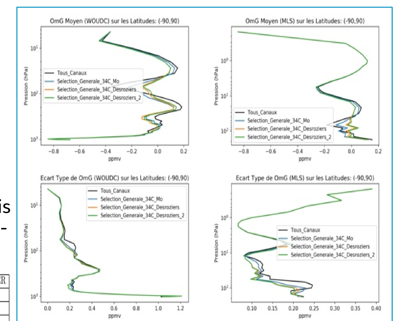
Fig 6: Vertical profiles of scores wrt WUDC (left) and MLS (right), for biases (top) and standard deviations (bottom).
