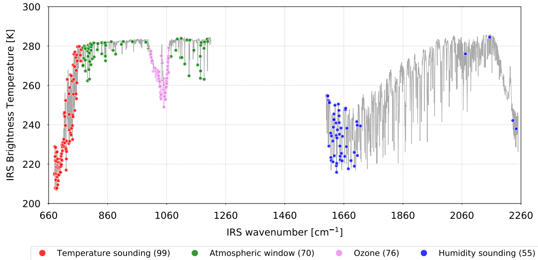
Figure 15. Location of the 300 selected IRS channels on a typical spectrum by main sensitivity.
