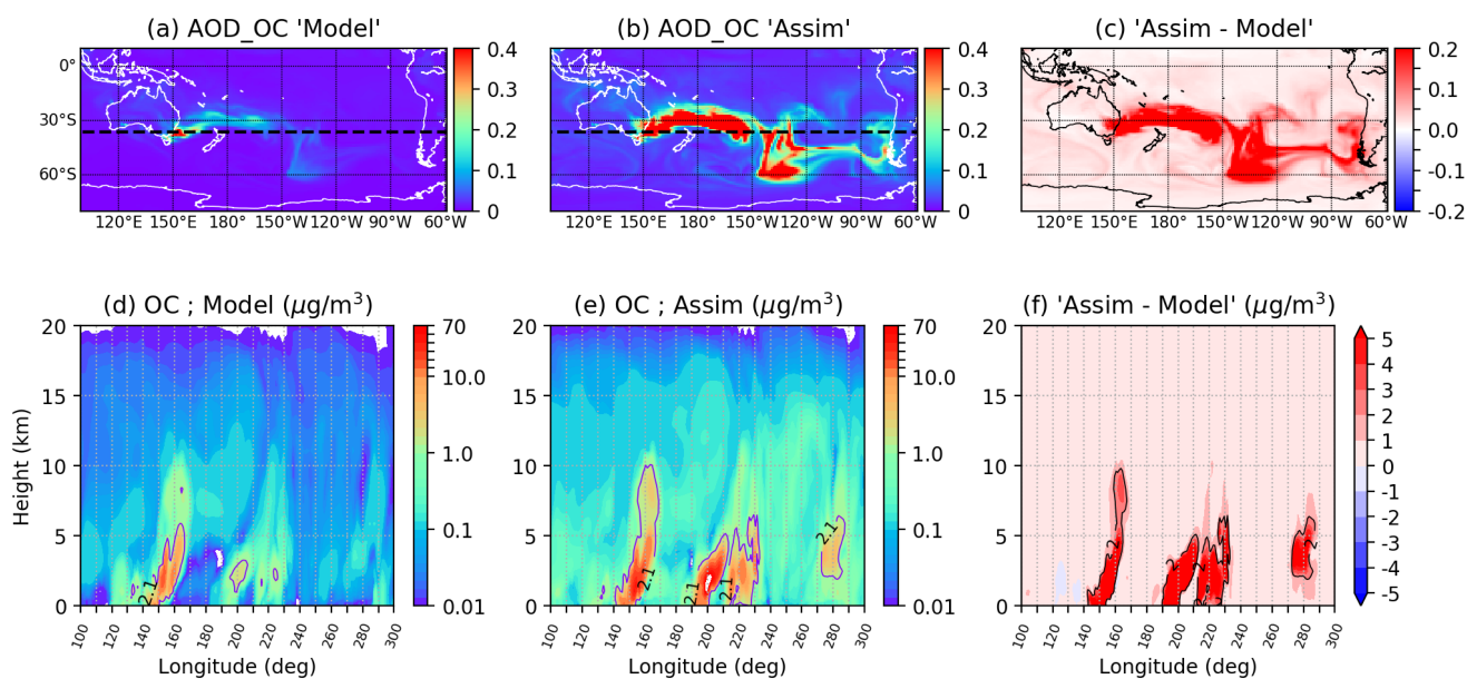
Figure 10. (Top): Aerosol Optical Depth of Organic Carbon (OC) over the Australian continent issued from the model free run (a) and the MODIS assimilated field (b) for 6 January 2020. The difference between (b) and (a) is presented in (c). (d) The zonal cross-section of OC concentration issued from the model free run at 37.5°S between 110° and 300° in longitude and between 0 and 20 km in the vertical. Part (e) is the same as (d) but for the MODIS assimilated field. The differences between the assimilation and the model free run fields are presented in (f).
