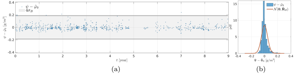
Figure 15. (a) Differences (\psi - \hat{\varphi}_0) ( \bullet ) superimposed on 4\sigma_B in shaded gray, and (b) normalized histograms of (\psi - \hat{\varphi}_0) and the pdf of B \sim \mathcal{N}(\mathbf{0}, \hat{\mathbf{R}}_B) .
