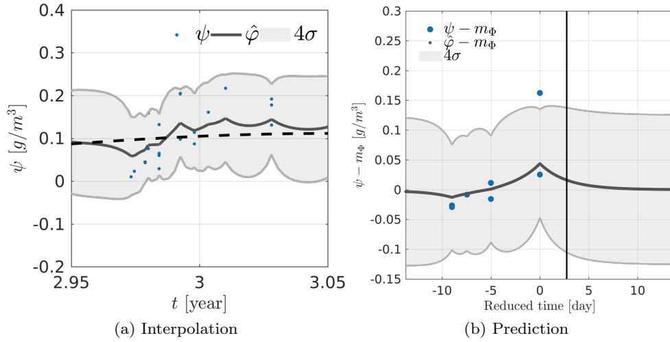
Figure 13. (a) Kriging based interpolation over a period of 36 days centered at the beginning of 3-rd in the dataset. The mean is represented in as a dashed black line (—). (b) Kriging based prediction over a period of \sim 36 days centered at the beginning of 3-rd in the dataset. The vertical black line (|) represents the correlation time l_t after the last observation. In (a) and (b), the training set observations are represented as (•), the kriging estimate as black line (—), and the variance of the estimation error in shaded gray.
