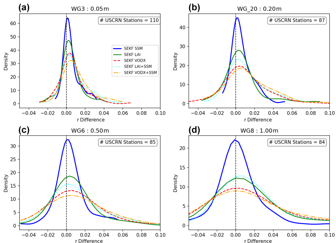
Figure 9. Probability distribution functions of the distribution of correlation differences between the OL and SEKF SSM (solid bold blue line), SEKF LAI (solid green line), SEKF VODX (dashed red line), SEKF LAI SSM (dotted cyan line), and SEKF VODX SSM (dash-dotted orange line) for USCRN at (a) WG3 (5 cm), (b) WG_20 (20 cm), (c) WG6 (50 cm), and (d) WG8 (100 cm) between 2011 and 2018.
