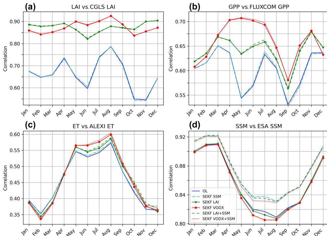
Figure 10. Graphs of monthly correlations over CONUS between the LDAS-Monde OL (solid blue line), SEKF SSM (dash-dotted cyan line), SEKF LAI (solid green line with star markers), SEKF VODX (solid red line with cross markers), SEKF LAI SSM (dashed green line), and SEKF VODX SSM (dotted red line) and satellite-derived observations of (a) LAI (2003 to 2018), (b) GPP (2003 to 2013), (c) ET (2003 to 2018), and (d) SSM (2003 to 2018).
