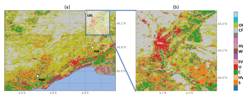
Figure 3. Land cover (CGLS) for (a) the Montpellier region and for (b) the Alès sub-domain ( 4^{\circ} – 4.3^{\circ}E , 43.95^{\circ} – 44.25^{\circ}N ), including the city of Alès. Land cover classes: open forest (“OF”), closed forest (“CF”), herbaceous wetland (“HW”), permanent water bodies (“WB”), sparse vegetation (“SV”), urban (“U”), cropland (“C”), herbaceous vegetation (“HV”), and shrubs (“S”). “OF” and “S” may include crop fields, vineyards, and orchards. The locations of the Pezenas, La Grand Combe, and Villevieille SMOSMANIA stations (PZN, LGC, and VLV, respectively) are shown.
