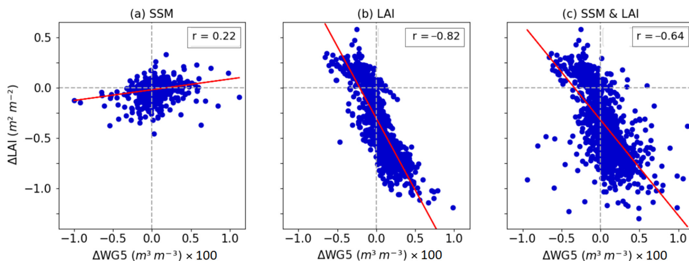
Figure 11. Year-to-year evolution from 2018 to 2019 over the Alès sub-domain of the mean differences in July between analyzed and open-loop LAI vs. the mean differences in July between analyzed and open-loop WG5 between (a) S1 SSM assimilated alone, (b) PROBA-V LAI assimilated alone, and (c) SSM and LAI jointly assimilated.
