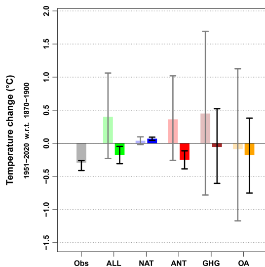
Figure 2. Changes induced by various subsets of external forcings over the historical period (1951–2020 with respect to (w.r.t.) 1870–1900) over the warming hole. Observed (Obs) changes (gray, left) are deduced from HadSST4 observations; uncertainty only includes observational uncertainty (i.e., measurement and processing; internal variability is ignored). For all other contributions, the bar and gray confidence interval on the left-hand side describe the DAMIP model range, assuming a Gaussian distribution. The bar and black confidence interval on the right-hand side correspond to results constrained by observations. All ranges shown are 5% to 95% confidence ranges. The SSP2-4.5 scenario is used to extend historical simulations after 2014.
