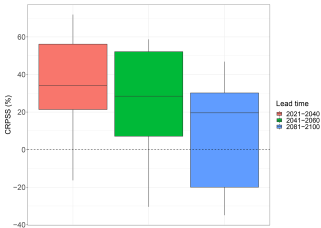
Figure 4. CRPSS for the constrained SST projections over the WH within the perfect model framework. The red, green and blue box-plots indicate the CRPSS distributions for different lead times. Calculation is made for all CMIP6 ensemble members (see Table A1). The top (bottom) of the box represents the 25th (75th) percentile of the distribution and the upper (lower) whisker represents the 95th (5th) percentile. Values are normalized by the number of members in each model. A CRPSS of 0 (dashed line) indicates the absence of added values of the method.
