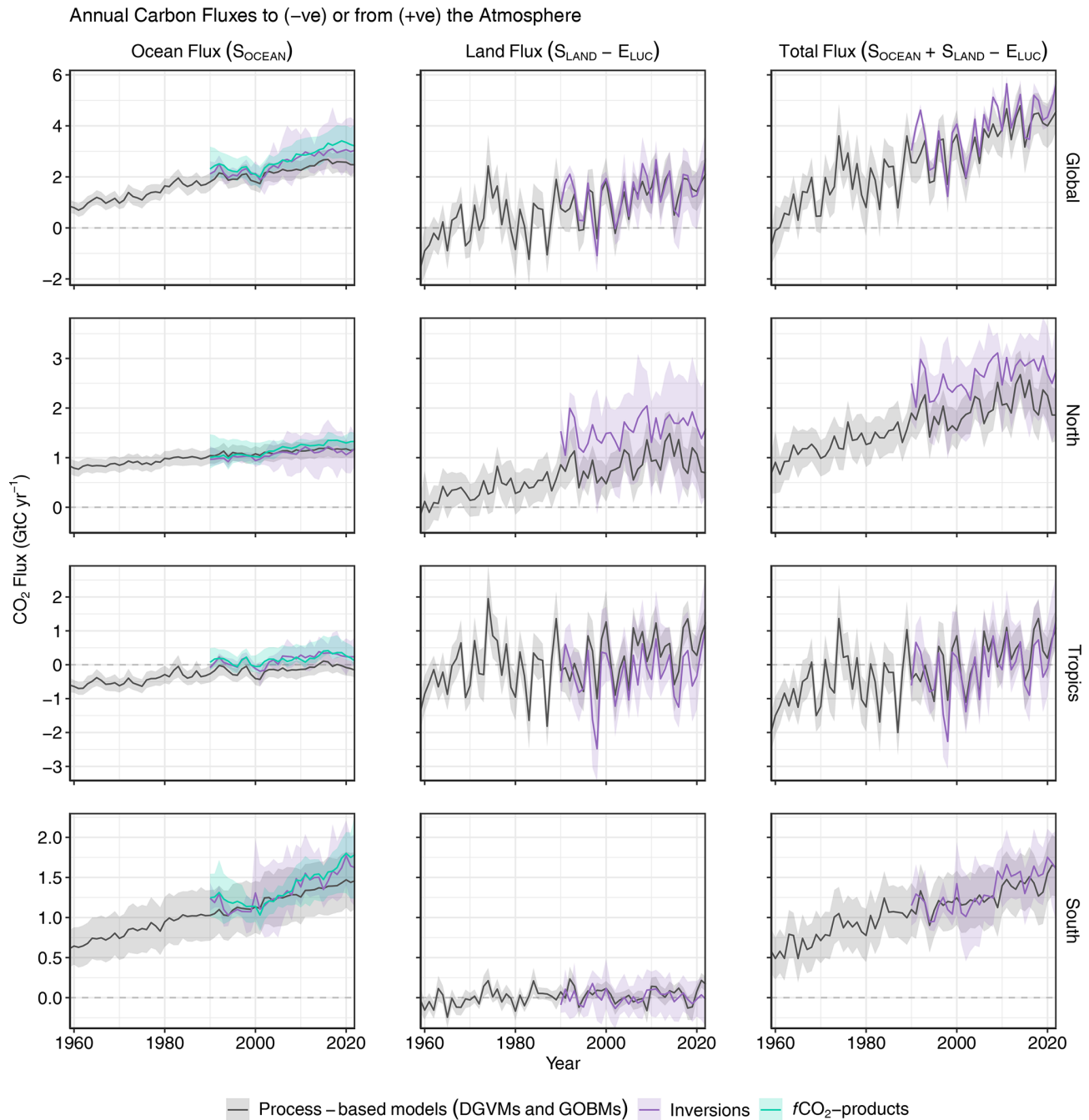
Figure 13. \text{CO}_2 fluxes between the atmosphere and the Earth’s surface separated between land and oceans, globally and in three latitude bands. The ocean flux is S_{\text{OCEAN}} , and the land flux is the net atmosphere–land fluxes from the DGVMs. The latitude bands are (top row) global, (second row) north ( > 30^\circ \text{N} ), (third row) tropics ( 30^\circ \text{S}–30^\circ \text{N} ), and (bottom row) south ( < 30^\circ \text{S} ). The fluxes are over ocean (left column), over land (middle column), and total (right column). Estimates are shown for the following: process-based models (DGVMs for land, GOBMs for oceans), inversion systems (land and ocean), and f\text{CO}_2 products (ocean only). Positive values are \text{CO}_2 sinks. Mean estimates from the combination of the process models for the land and oceans are shown (black line) with \pm 1\sigma of the model ensemble (grey shading). For the total uncertainty in the process-based estimate of the total sink, uncertainties are summed in quadrature. Mean estimates from the atmospheric inversions are shown (purple lines) with their full spread (purple shading). Mean estimates from the f\text{CO}_2 products are shown for the ocean domain (light-blue lines) with their full model spread (light-blue shading). The global S_{\text{OCEAN}} (upper left) and the sum of S_{\text{OCEAN}} in all three regions represent the anthropogenic atmosphere-to-ocean flux based on the assumption that the pre-industrial ocean sink was 0 \text{ Gt C yr}^{-1} when riverine fluxes are not considered. This assumption does not hold at the regional level, where pre-industrial fluxes can be significantly different from zero. Hence, the regional panels for S_{\text{OCEAN}} represent a combination of natural and anthropogenic fluxes. Bias correction and area weighting were only applied to global S_{\text{OCEAN}} ; hence the sum of the regions is slightly different from the global estimate ( < 0.05 \text{ Gt C yr}^{-1} ).
