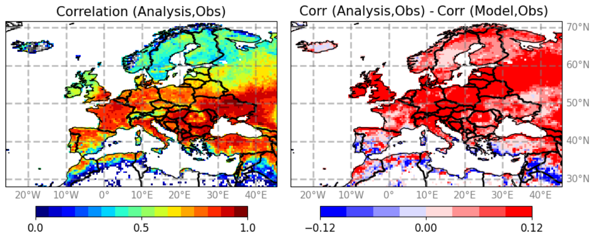
Figure 6: Correlation maps between the TROPOMI SIF observations and the LAI analysis for the 2018–2020 period (left column) and the difference map (right column, where red means an improvement after assimilation).
