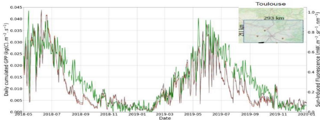
Figure 4: Daily time series of S5-P SIF and OL_EUMED and SEKF_LAI_EUMED GPP (green, dark, and red lines, respectively) over the region of Toulouse in France from 1 May 2018 to 31 December 2019.
