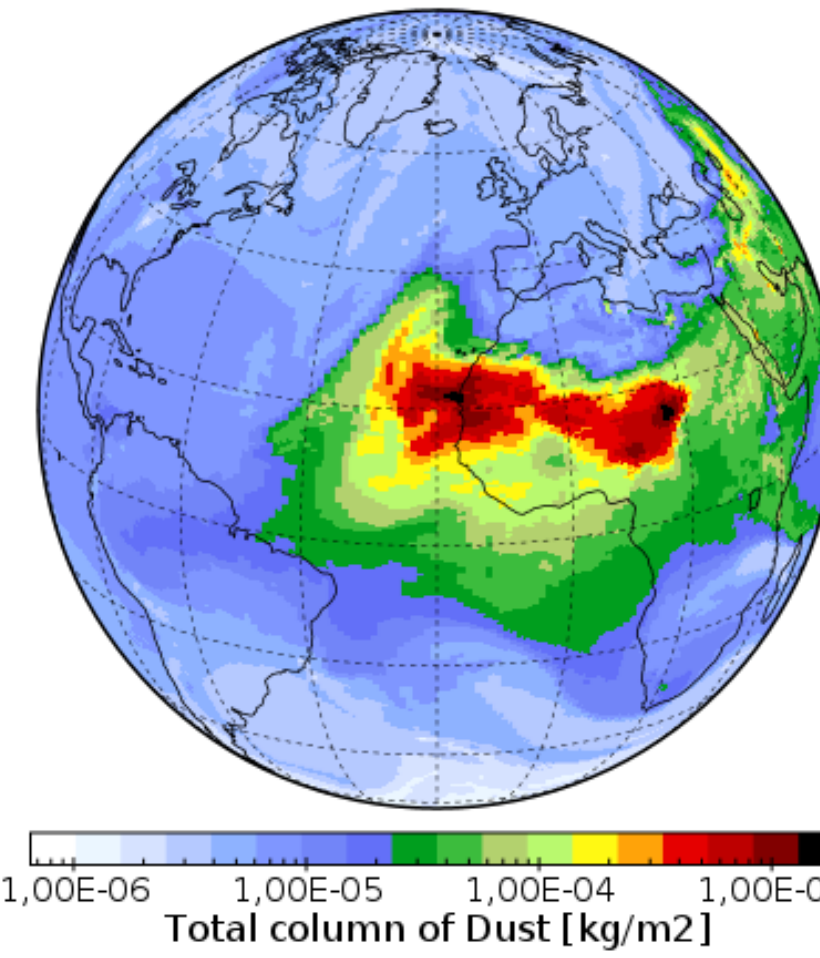
Fig.2 Total dust column on January 24, 2024 at 12 UTC
