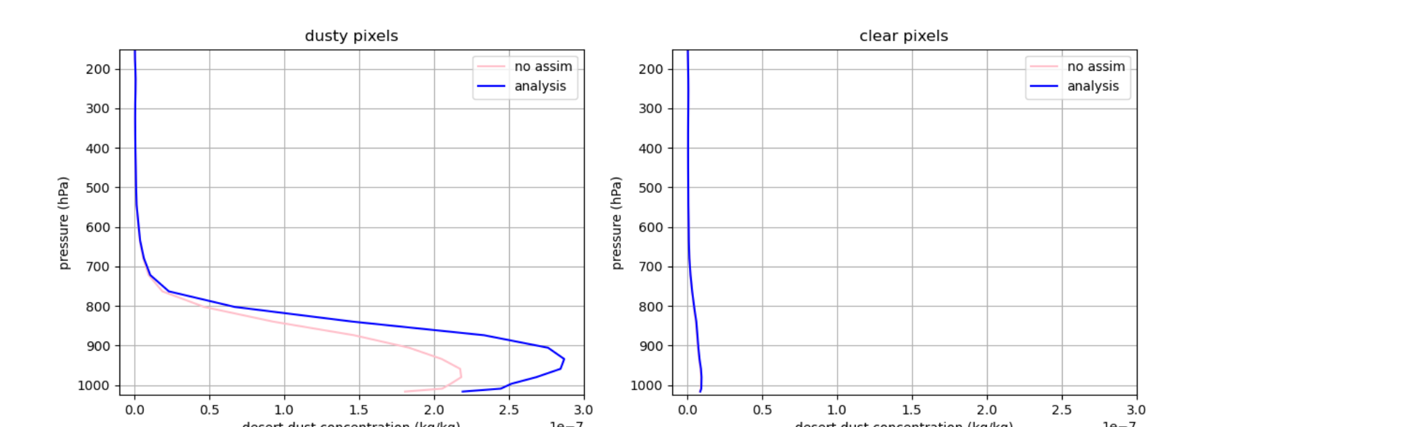
Fig.9 Average profiles of desert dust concentration, with no assimilation (pink) and IASI assimilation (blue), for dusty pixels (left) and clear pixels (right), for 25 January 2024
