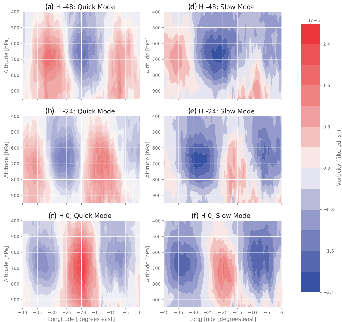
FIGURE 11 Longitude–height cross-section of vorticity composites for (a–c) quick-mode trajectories and (d–f) slow-mode trajectories. The time reference for compositing (H0) is taken when the tracked AEW crosses 20°W, at the latitude at which the trajectory crosses 20°W. The vertical structure is shown (a,d) 48 h prior to AEWs crossing 20°W, (b,e) 24 h prior to AEWs crossing 20°W, and (c,f) at the time AEWs cross 20°N.
