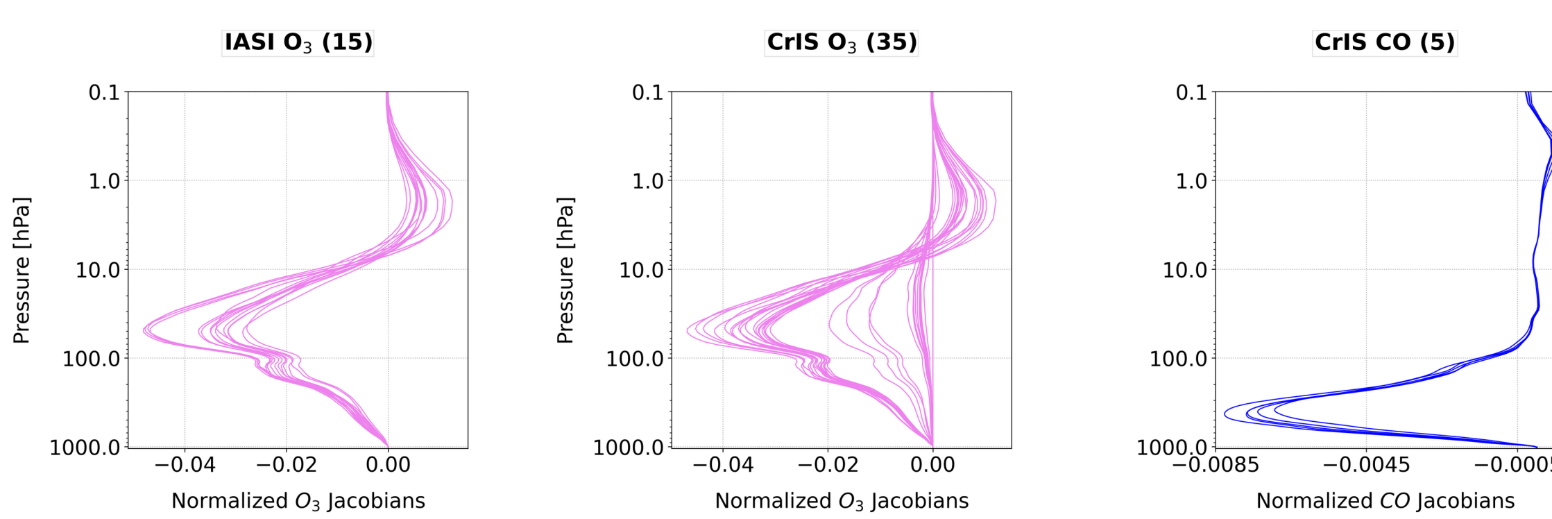
Fig.3 Normalized jacobians for 15 IASI ozone-sensitive channels (left), 35 CrIS ozone-sensitive channels (middle) and 5 carbon monoxide-sensitive channels (right)
