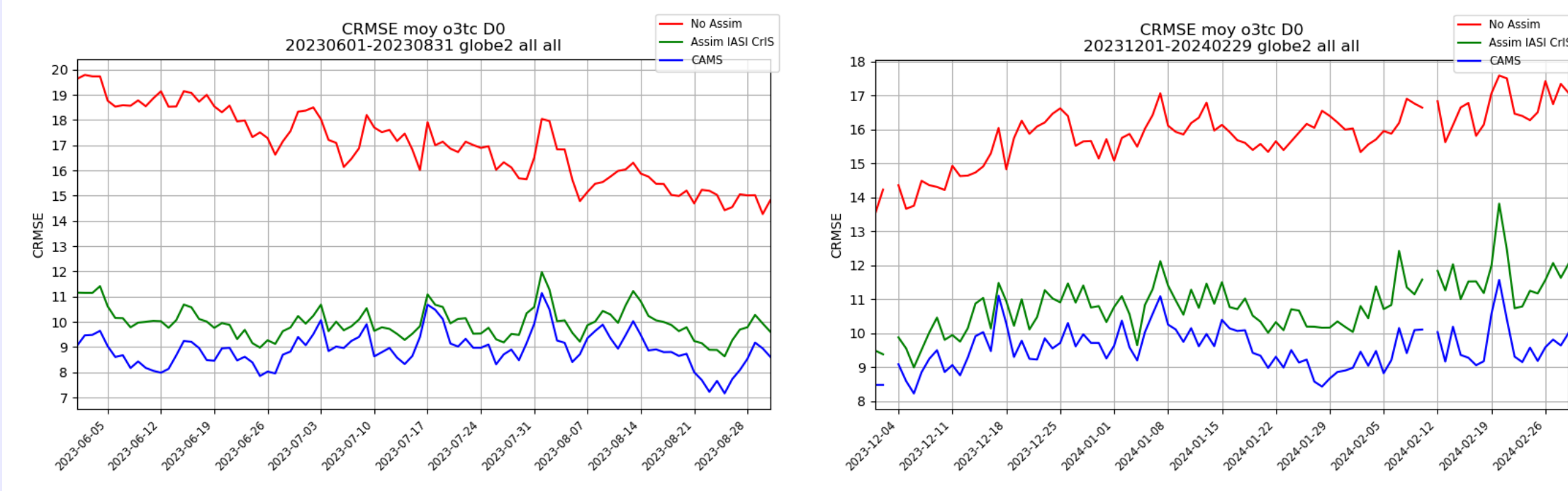
Fig.8 Temporal CRMSE on the globe for experiments without assim (red) with assim (green) and for CAMS (blue) wrt. OMI ozone total column for 3 summer months (left) and 3 winter months (right).
