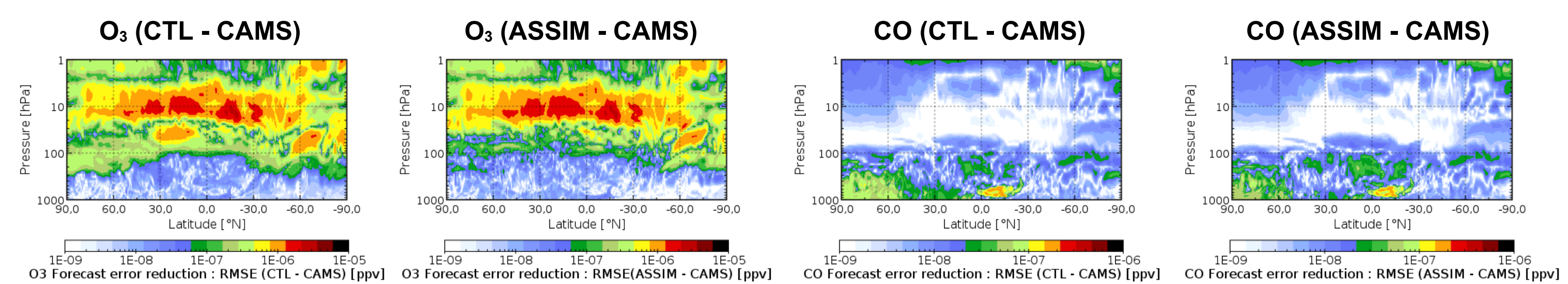
Fig.10 Forecast error reduction (RMSE) on the atmospheric vertical as a function of latitude (at 0° longitude) for the 3 months of summer period (JJA) for the ozone (left) and carbon monoxide (right) fields of the control experiment and the IASI-CrIS assimilation experiment compared with the CAMS forecasts.
