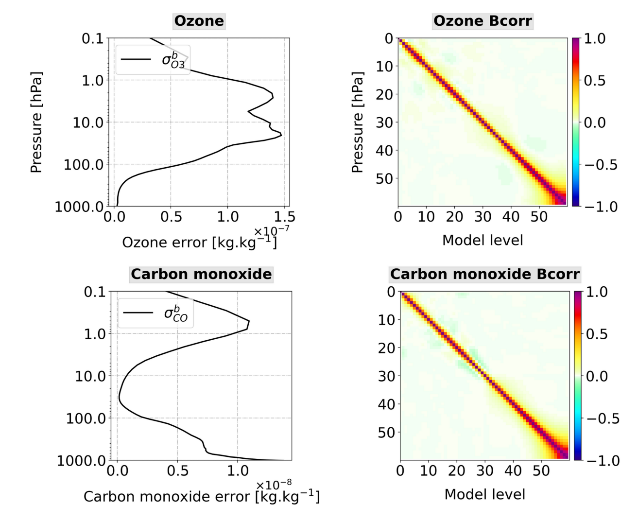
Fig.5 Background error standard deviation of ozone on the atmospheric vertical (pressure) and associated vertical error correlations (levels) (top) and same for carbon monoxide (bottom).
