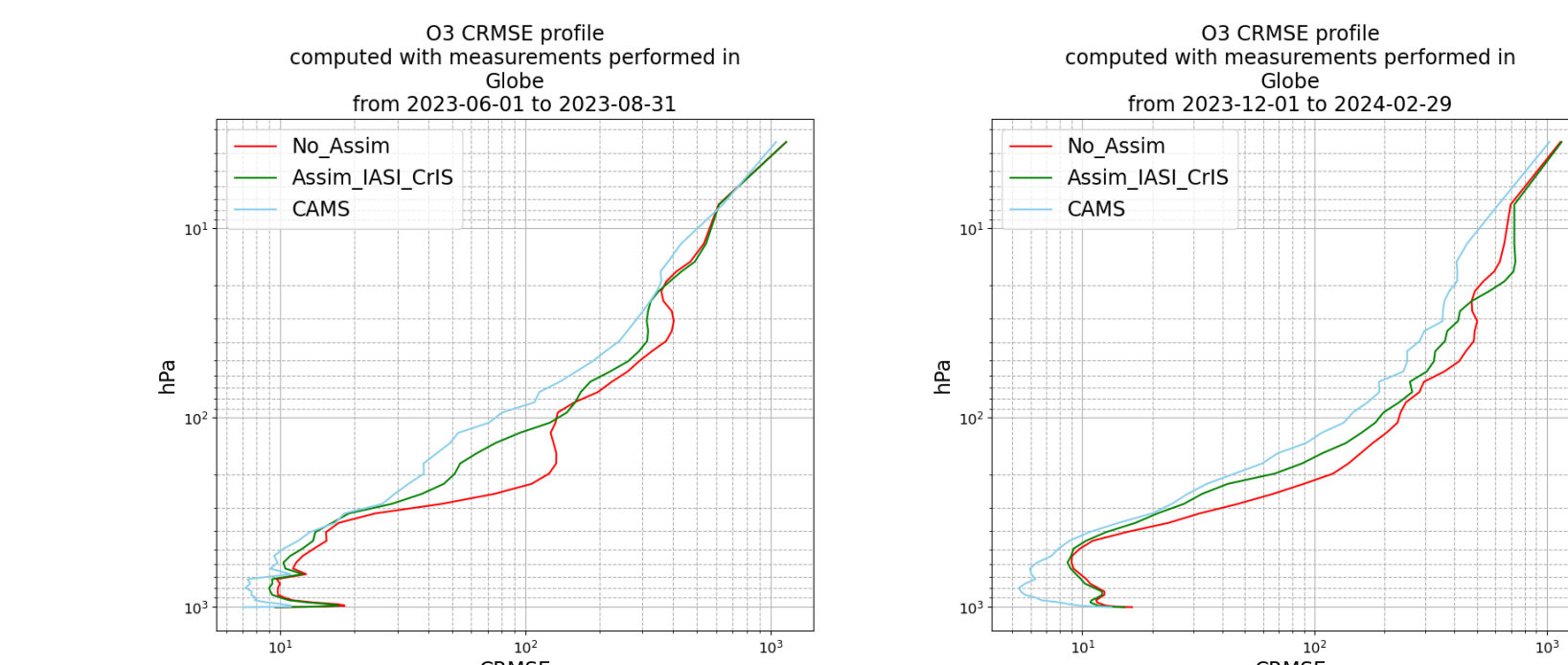
Fig.7 CRMSE on the globe for experiments without assim (red) with assim (green) and for CAMS (blue) wrt. ozonesondes for 3 summer months (left) and 3 winter months (right).
