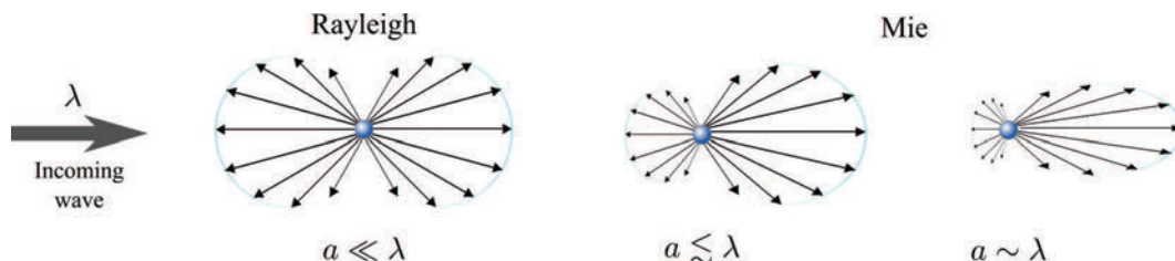
Figure 3.1 – Mie and Rayleigh directions of backscatter.
